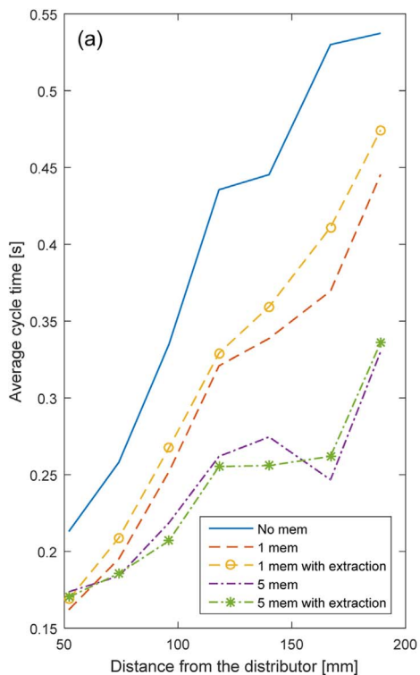
Fig. 14. (a) Average cycle time and (b) average amplitude of the output signal at different axial positions along the reactor (for all the cases the inlet velocity was corrected for membrane (s) presence and gas extraction to keep the outlet velocity at U/U_{mf} = 2 . Each point in the graphs represents the average of 2100 frames (at 35 Hz) over a pixel pocket of 50 \times 50 at r/R = 0.5 .
