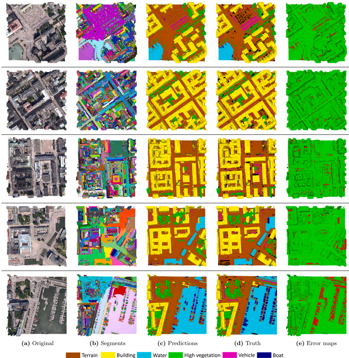
Fig. 12. Part of our semantic segmentation results. The first column shows the input texture meshes; the second column shows the over-segmentation results; the third column shows the predicted semantic meshes; the fourth column shows the ground truth meshes; the last column shows the error maps (red: errors; green: correct labels). (For interpretation of the references to colour in this figure legend, the reader is referred to the web version of this article.)
