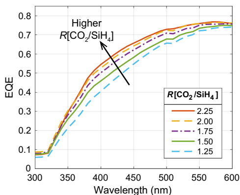
Fig. 2. EQE of a-SiGe:H cells with p-layers deposited at different concentration of CO 2 . The spectra were measured at bias voltage V_{\text{bias}} = -0.5 V, to feature the optical effect.
