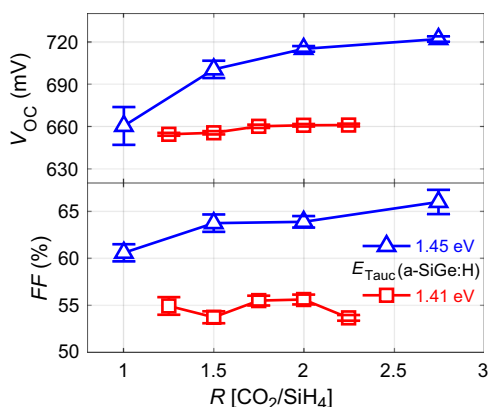
Fig. 3. External parameters V_{\text{OC}} and FF of a-SiGe:H cells with p-SiO x :H made with different ratio of R[\text{CO}_2/\text{SiH}_4] .
