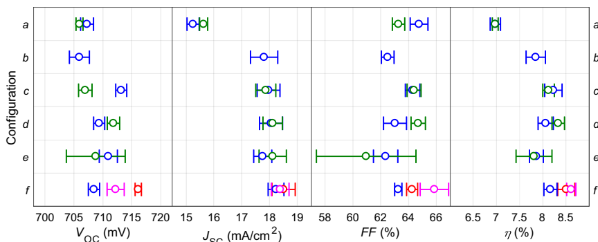
Fig. 4. External parameters of a-SiGe:H cells with different configurations of the n-layer. The multiple data sets (different colors) in a configuration represent samples having the same nominal structure but made in different deposition runs. The error bars are the standard deviation showing the inhomogeneity among the cells within a sample. (For interpretation of the references to color in this figure legend, the reader is referred to the web version of this article.)
