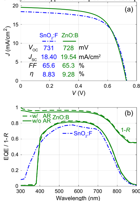
Fig. 6. (a) Current density-voltage ( J - V ) curves acquired under AM1.5G illumination, and (b) EQE measured at short-circuit condition, of the optimized a-SiGe:H cells fabricated on substrates with different light-scattering capability. Additionally, the EQE and 1- R spectra are given for the cells on ZnO:B substrate with (w/) and without (w/o) anti-reflection treatment.
