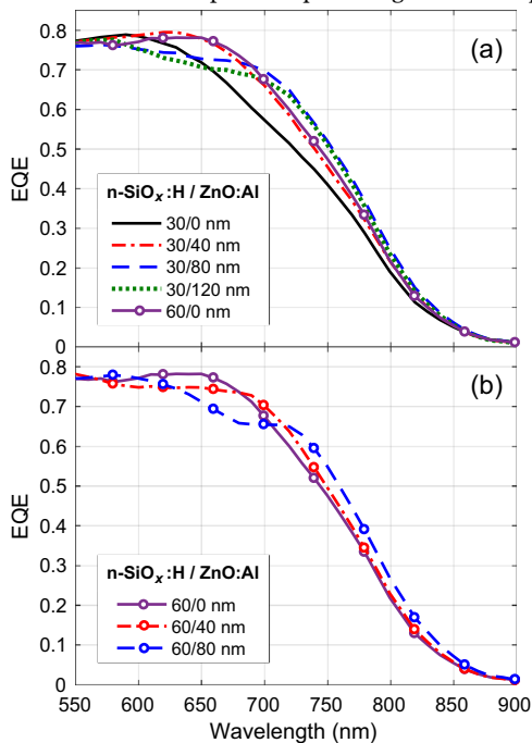
Fig. 5. EQE of a-SiGe:H cells with different thicknesses of n-SiO x :H and ZnO:Al in front of the back reflector. The thickness of n-SiO x :H is (a) 30 nm or (b) 60 nm in total. The result of the cell with 60-nm-thick n-SiO x :H and no ZnO:Al is also plotted in (a) to show
