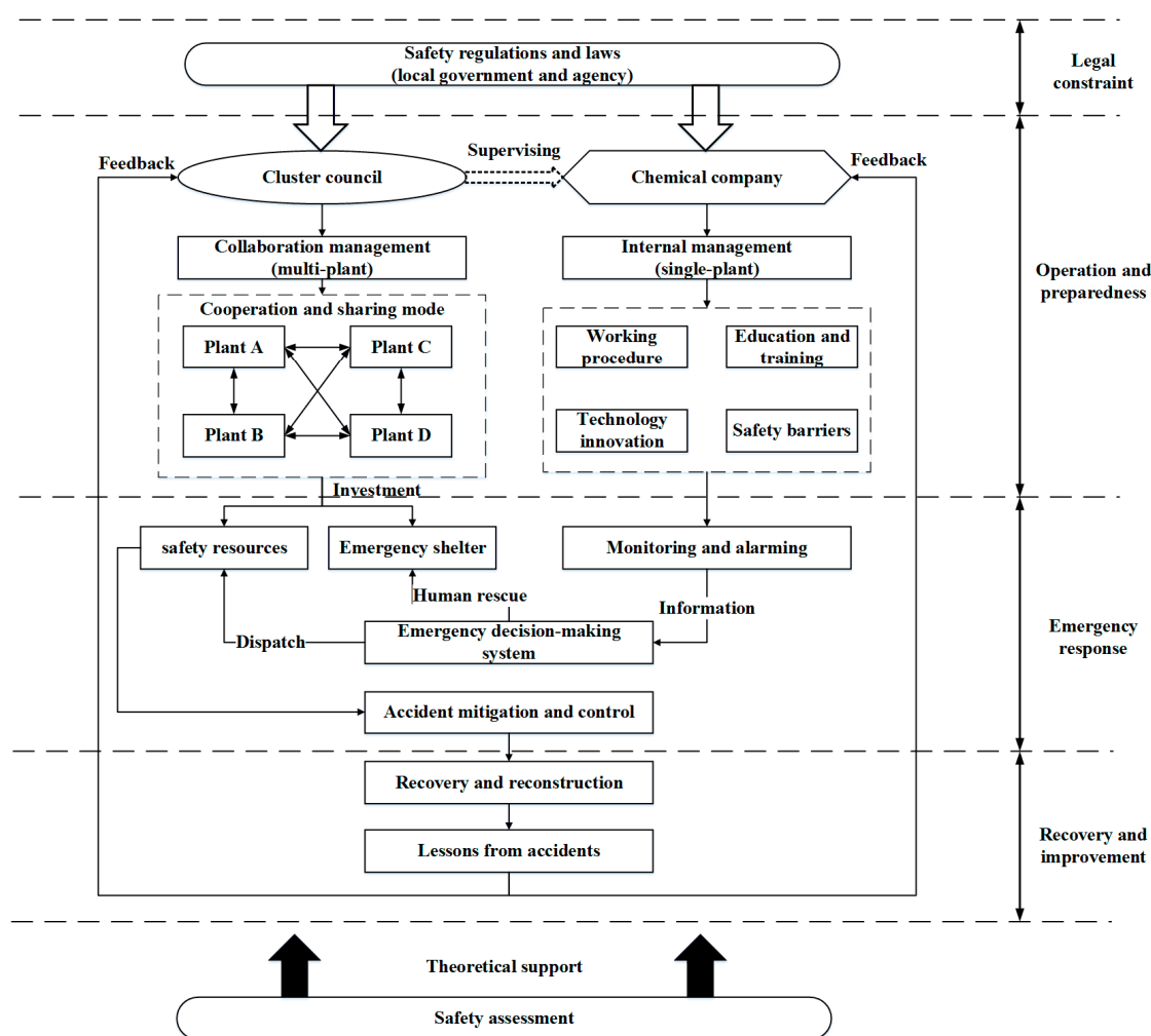
Figure 6. The integrating safety framework for CIP.
