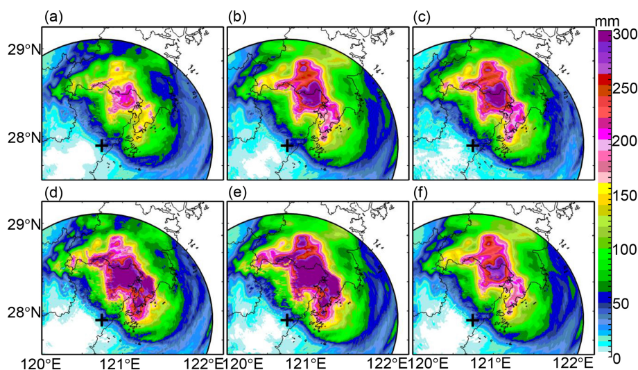
Figure 21. The 6 h rainfall estimates derived from (a) R(Z_H^M) , (b) R(Z_H^C) , (c) R(K_{DP}) , (d) R(Z_H^M, Z_{DR}^M) , (e) R(Z_H^C, Z_{DR}^C) , and (f) R(Z_H^C, \hat{Z}_{DR}) at 22:00 UTC, 9 August 2019. Two dashed lines refer to the GWS of YDM and KCM, and + refers to the WZ-SPOL radar site.
