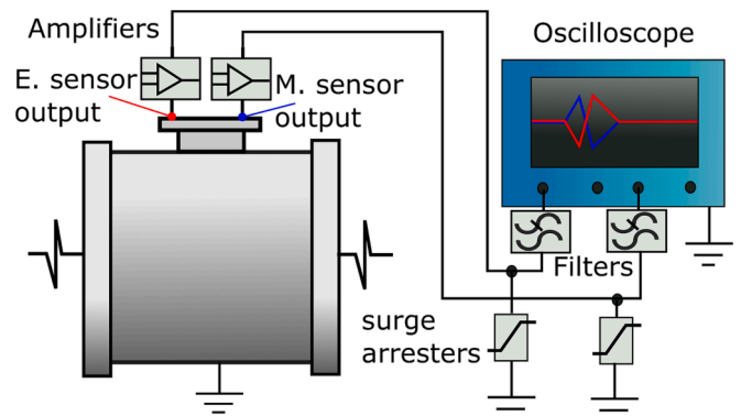
Fig. 10. Measuring system used for the testbench and the full-scale GIS. The surge arresters were not used in the testbench.
