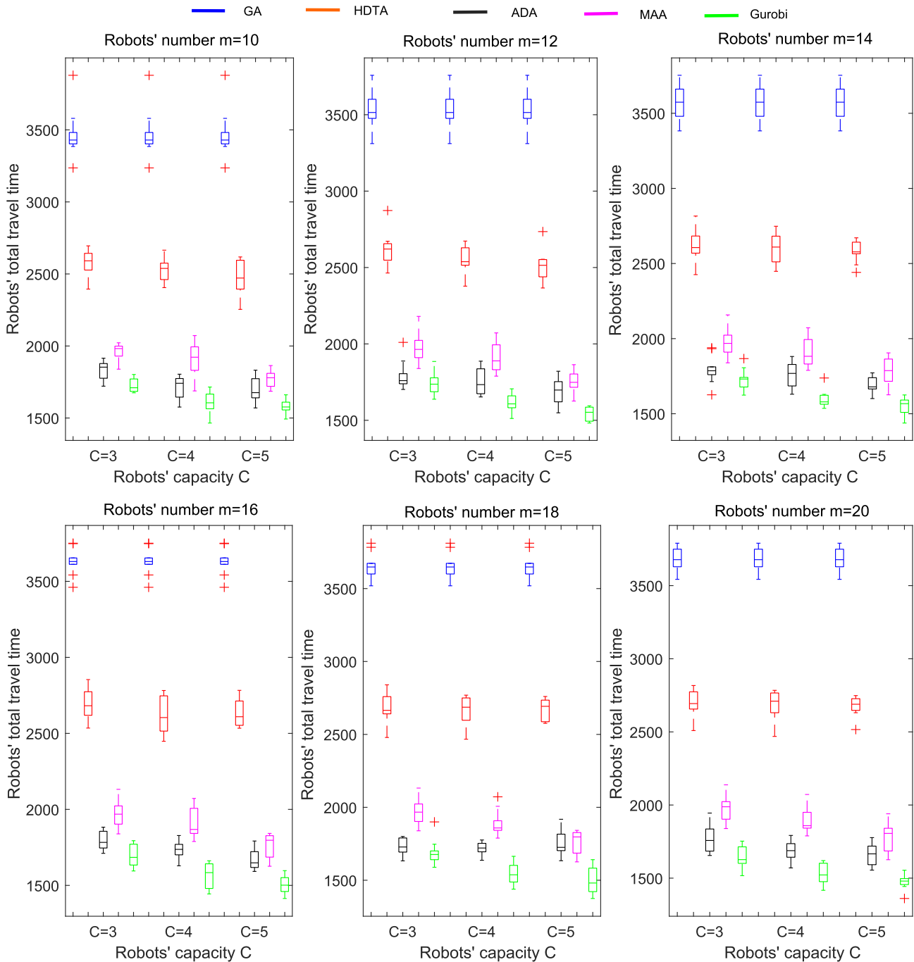
Fig. 2. Box plots of the robots' total travel times (s) under 10 instances to transport 100 dynamically released packages with different numbers of robots and different capacities, where the maximum time-delay for transporting each package is 8 minutes.
