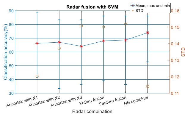
Fig. 5. The statistical parameters (classification accuracy in percentage and standard deviation of the values) for individual radar sensors and different fusion techniques using classifier SVM.
