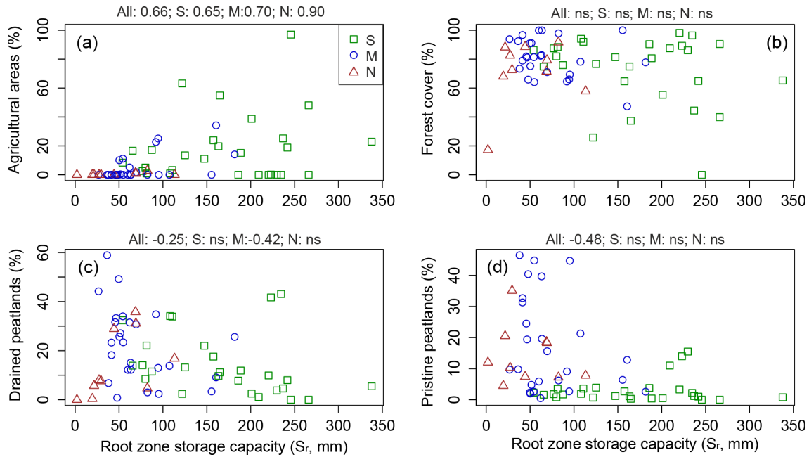
Figure 7. Root zone storage capacities ( S_r , mm) and proportion of (a) agricultural areas (%), (b) forest cover (%), (c) drained peatlands (%) and (d) undrained peatlands (%) in the catchment at different ecoregions (S is south boreal, M is mid-boreal and N is north boreal). The titles of the sub-plots show the Spearman's correlation coefficients (significant correlation for p < 0.05 ).
