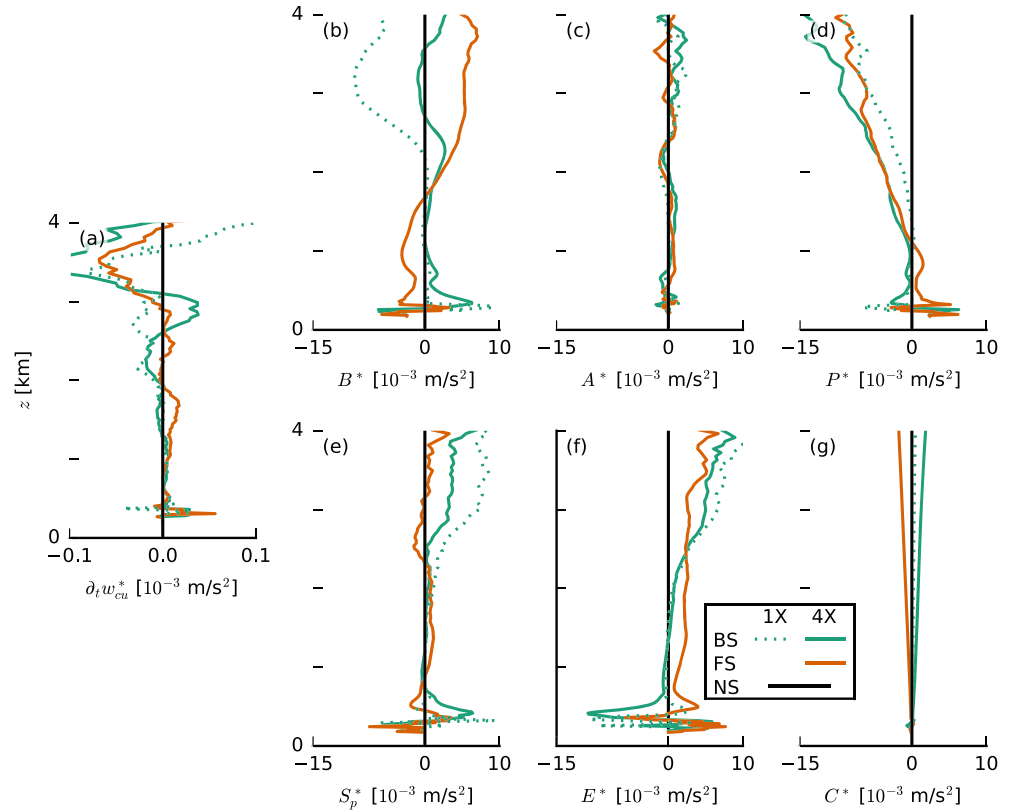
Figure A1. Slab-averaged profiles (averaged from 30 to 36 hr of the simulations with prescribed surface fluxes) of the terms of the cloudy-updraft vertical-velocity budget (Equation A1) plotted as differences from the NS case (indicated by the asterisks).
