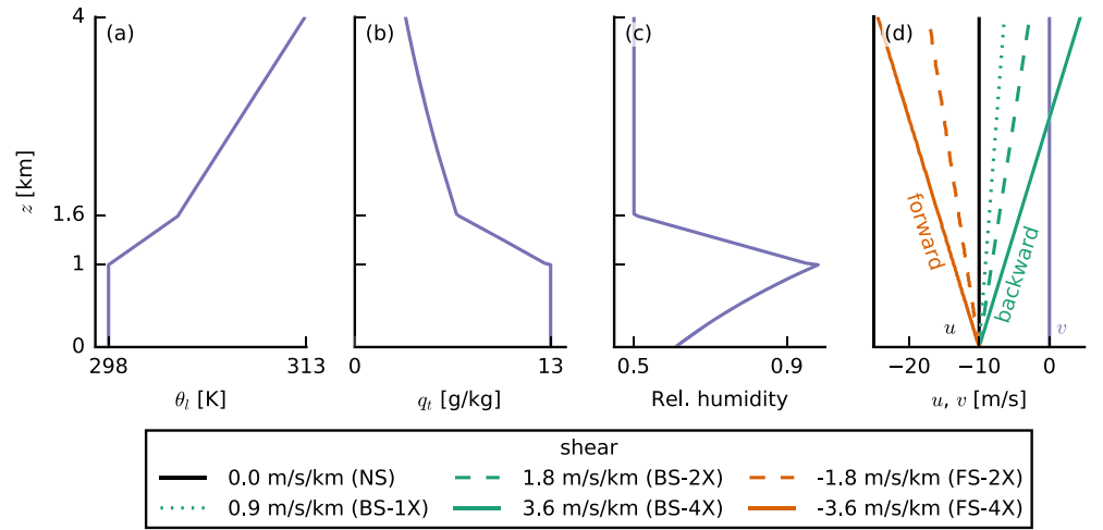
Figure 1. Initial profiles of (a) the liquid water potential temperature \theta_l , (b) total water specific humidity q_t , (c) relative humidity, and (d) the two wind components u and v . Purple profiles are the same in all simulations. Orange stands for forward shear (FS) and green for backward shear (BS). Same line types indicate the same amounts of absolute shear (1X, 2X, and 4X). The color coding of the different shears is the same for all other figures.
