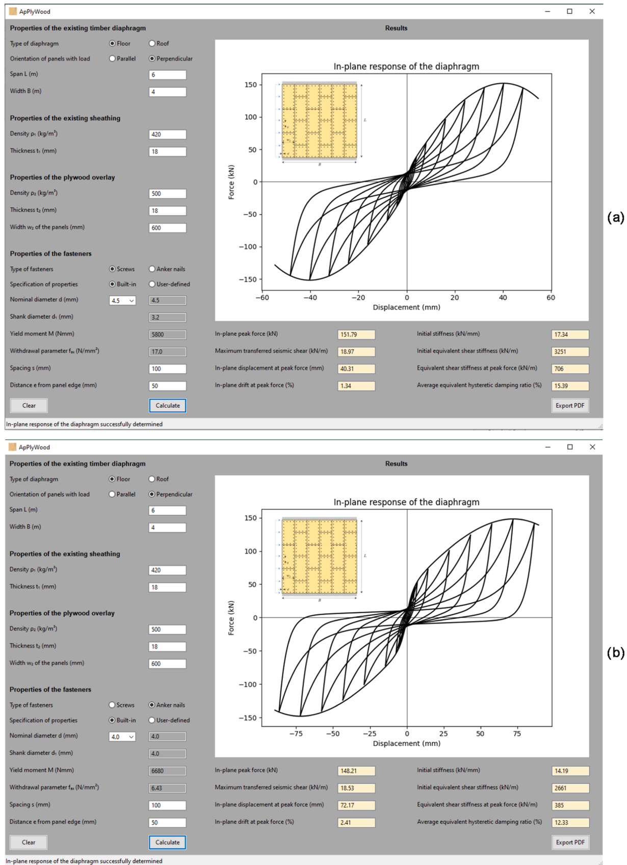
Fig. 12. Examples of calculated in-plane response from ApPlyWood to be used as input for the numerical model: floor retrofitted with plywood panels fastened with screws (a) or nails (b) to the existing sheathing.
