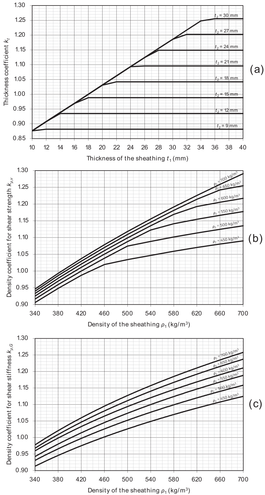
Fig. 7. Nomograms for coefficients k_t (a), k_{p,v} (b), and k_{p,G} (c) of Eqs. 4 and 5, referred to screws.
