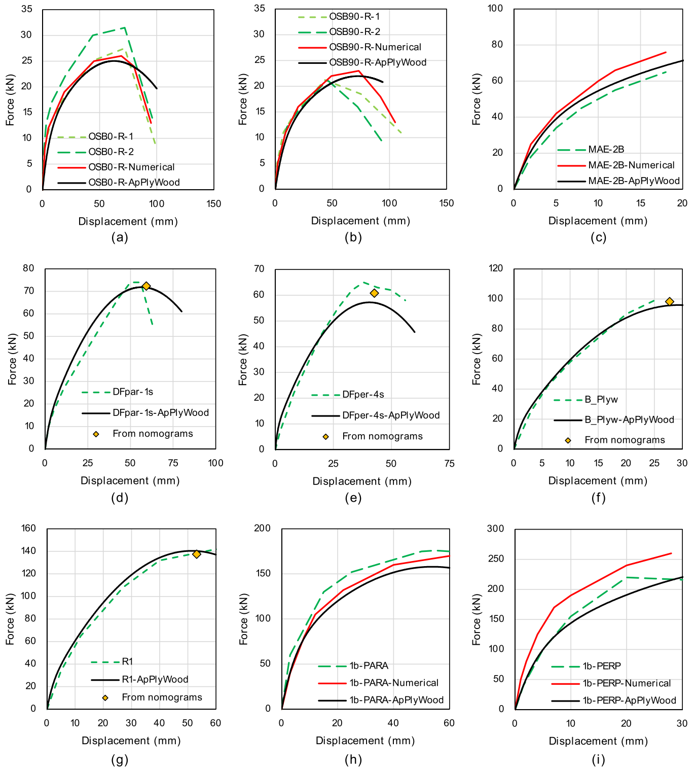
Fig. 10. Comparison between the outcomes from ApPlyWood calculation tool and the relevant selected studies from literature presented in Table 1: (a, b) experimental results and numerical analyses from Gubana and Melotto [7,52]; (c) experimental results from Peralta et al. [11,30] and numerical analyses from Masroor et al. [53]; (d, e) experimental results from Mirra et al. [15]; (f) experimental results from Rizzi et al. [14]; (g) experimental results from Brignola et al. [12]; (h, i) experimental results from Wilson et al. [13] and numerical analyses from Rizzi et al. [14]. For the diaphragms strengthened with plywood panels screwed to the existing sheathing (d, e, f, g), also the values from the nomograms of Section 3.1 are reported.
