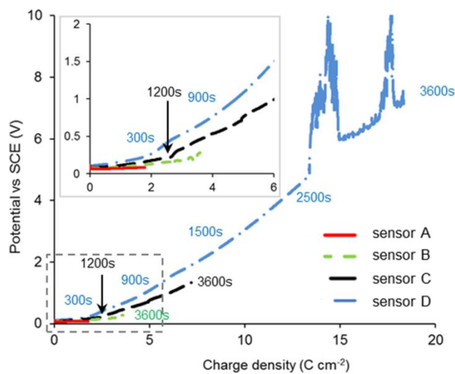
Figure 3.11: Overpotential vs. charge density during anodic formation of AgCl on a Ag wire in 0.1 M HCl in different current density regimes of 0.5 \text{ mA/cm}^2 (sensor A), 1 \text{ mA/cm}^2 (sensor B), 2 \text{ mA/cm}^2 (sensor C) and 4 \text{ mA/cm}^2 (sensor D).
