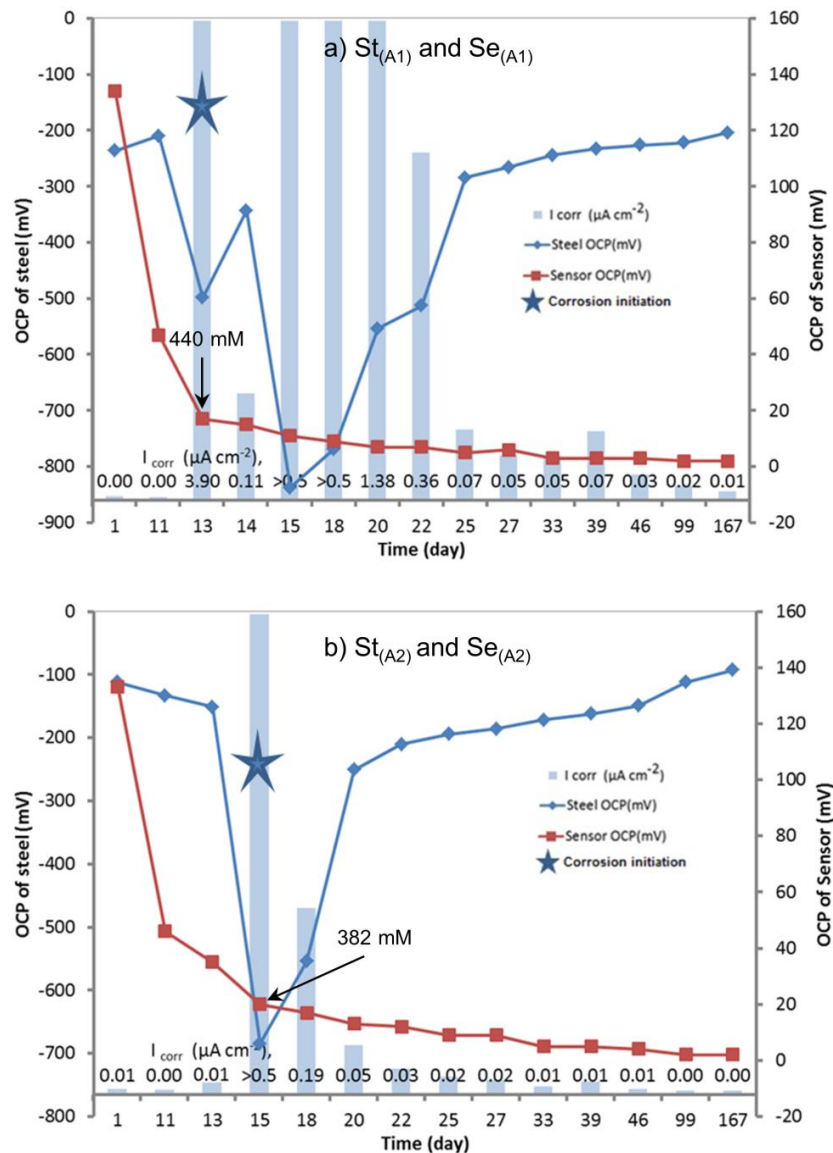
Figure 6.9: Corrosion current density ( I_{corr} ) of steel rods in addition to the OCP of steel and sensor at a certain time over immersion period: a) St_{(A1)} and Se_{(A1)} ; b) St_{(A2)} and Se_{(A2)}
