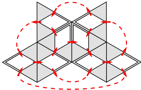
Fig. 7: The orientation of the triangular tiles on the net of the octahedron.
