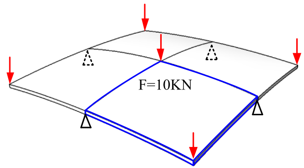
Fig. 12. The original shell.
