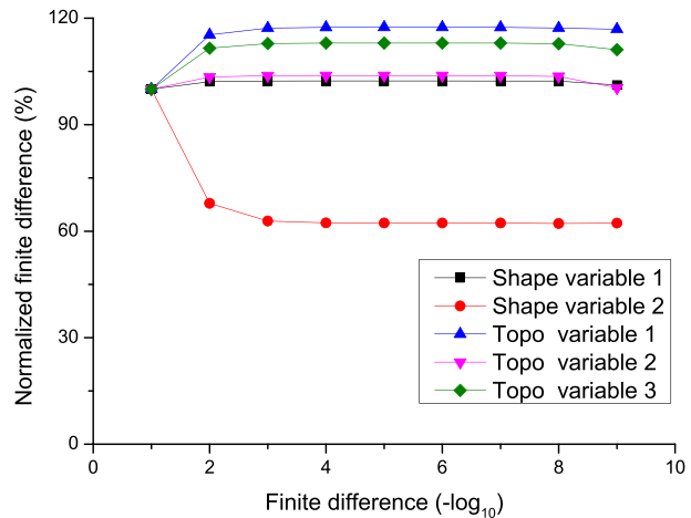
Fig. 13. Convergence analysis of the finite difference approximations.
