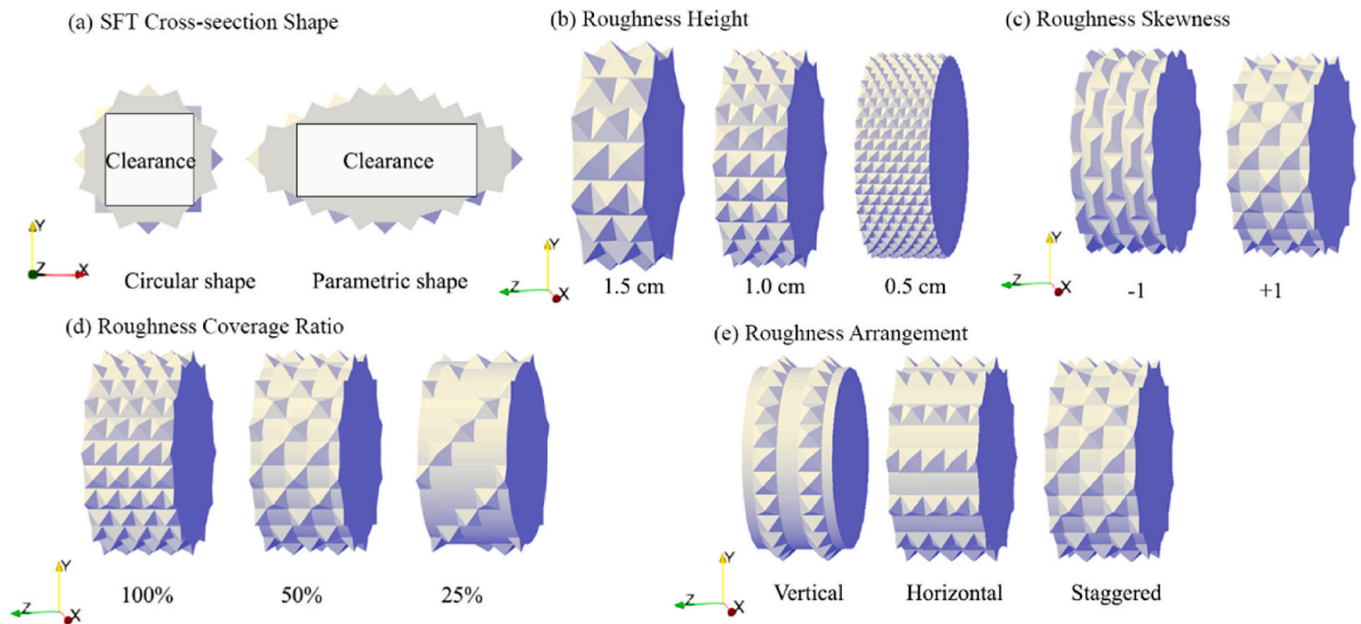
Fig. 4. SFT shapes and roughness parameters.
