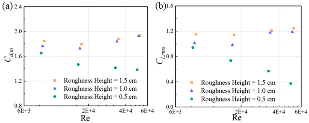
Fig. 11. Simulated hydrodynamic force coefficients for different roughness heights. (a) C_{d,m} vs Re ;(b) C_{l,rms} vs Re .
