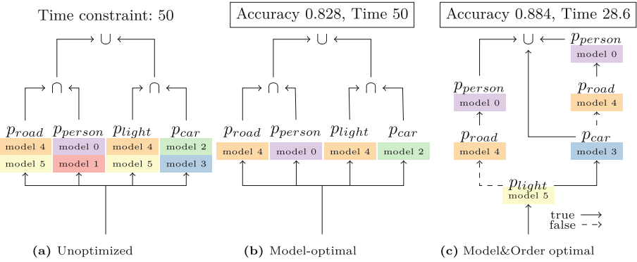
Fig. 1. Alternative ML query plans for the running example query.
