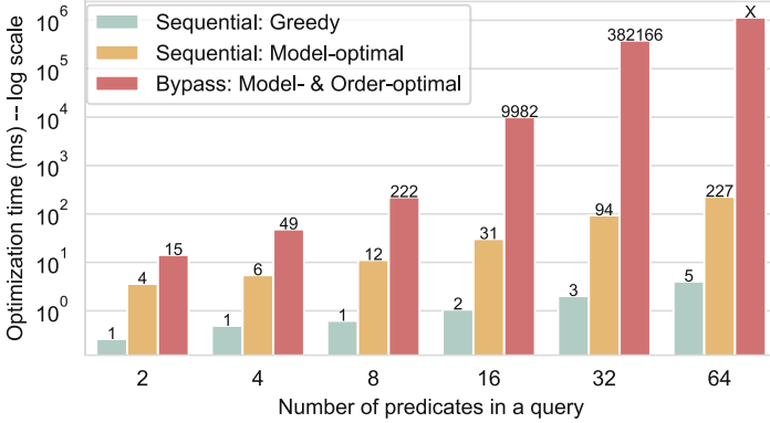
Fig. 6. Optimization time on queries with varying number of predicates.
