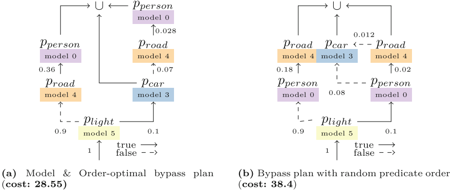
Fig. 3. Bypass plans with different predicate execution order (numbers near by the arrows indicating the selectivity of the predicates in that path).
