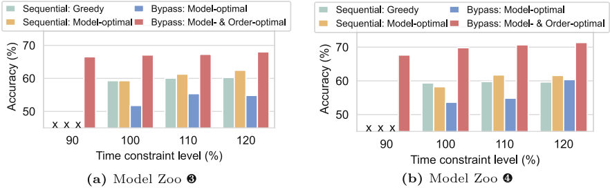
Fig. 5. The average accuracy on the query workload with different time (objective) constraint levels.
