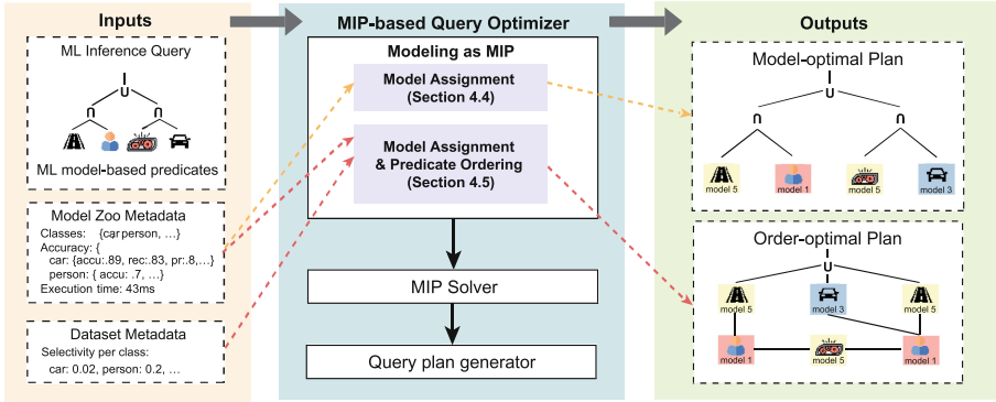
Fig. 2. Approach overview.
