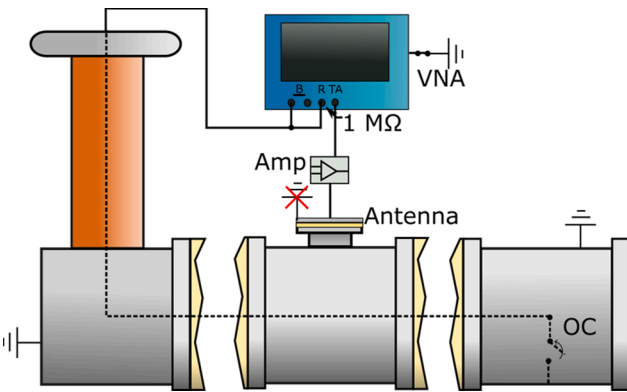
Fig. 6. Electric antenna calibration setup in a full-scale GIS.
