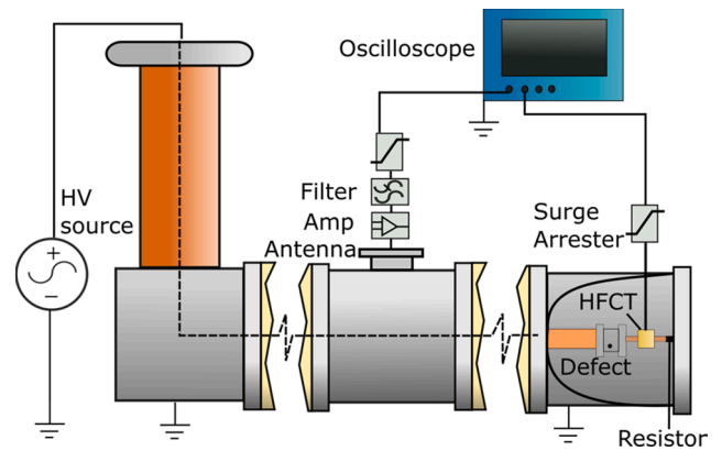
Fig. 12. Test setup for charge estimation in a full-scale GIS.
