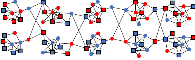
Fig. 7. The combined network is created by connecting five graphs (and their mirrors), whose individual cycle lengths are 17, 19, 21, 23 and 50. The combined network has a cycle length of lcm(17, 19, 21, 23, 50) = 7800450 .
