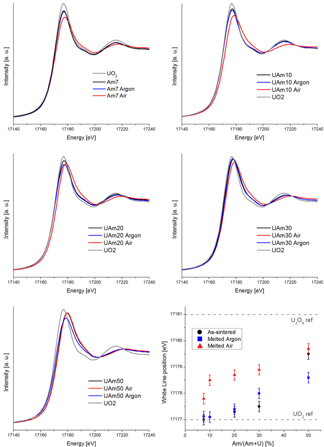
Fig. 9. XANES spectra collected at the U-L 3 edge on (U,Am)O 2-x , before and after melting. ( T = 298 \pm 5 K, P = 0.101 \pm 0.005 MPa). Bottom right: observed white lines.
