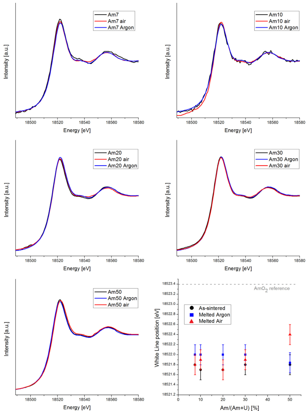
Fig. 8. XANES spectra collected at the Am-L 3 edge on (U,Am) 2-x F y , before and after melting. ( T = 298 \pm 5 K, P = 0.101 \pm 0.005 MPa). Bottom right: observed white lines.
