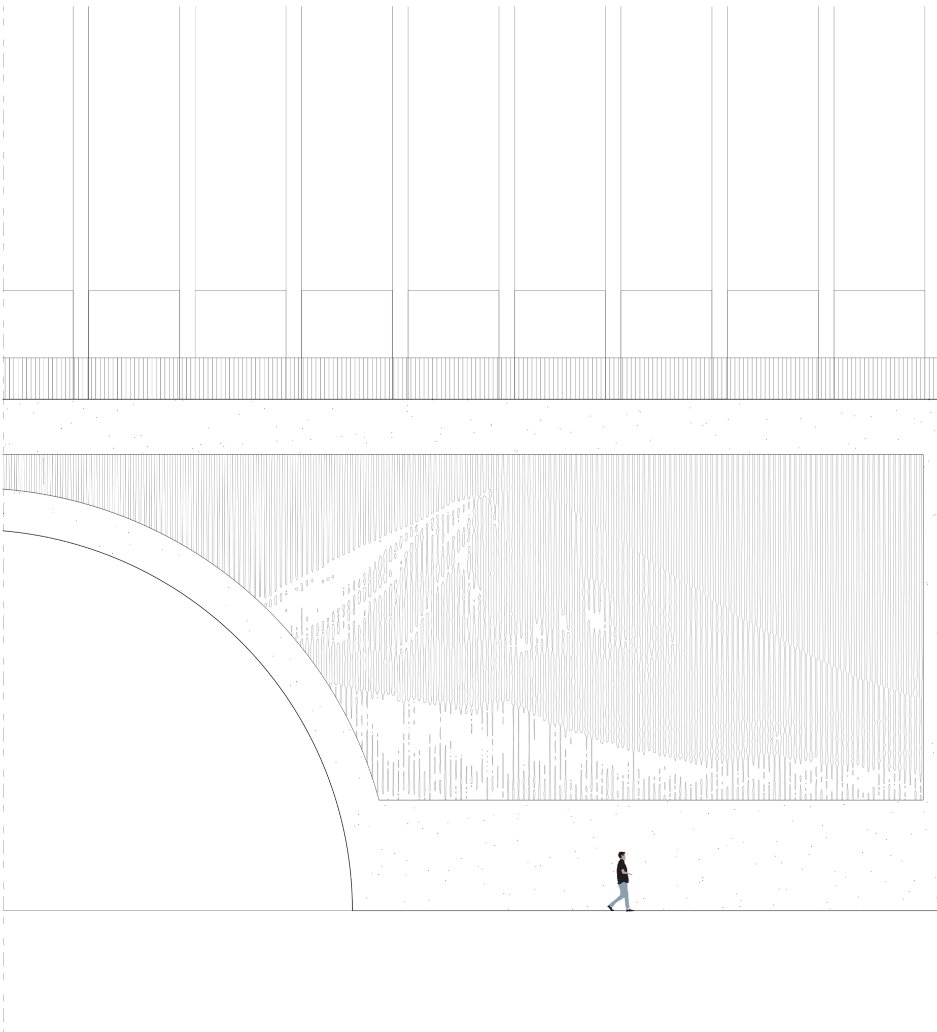
7 Cross-section and facade
