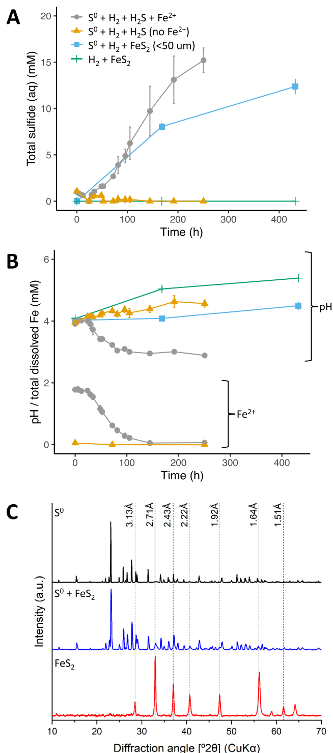
Figure 1. Total sulfide (mM) ( A ), total dissolved iron (mM) and pH ( B ), and XRD analysis of formed precipitates ( C ) in experiments carried out at 80 °C, starting pH 4. A. total sulfide concentrations in the liquid and gas phase expressed over the remaining liquid volume in experiments with mineral salts (MS) medium + S^0 , H_2 , H_2S supplementation (indicated with H_2S in the legend) and Fe^{2+} (grey circles); MS medium + S^0 , H_2 , H_2S supplementation but no Fe^{2+} (orange triangles); deionized water (DI) + S^0 , H_2 , and FeS_2 (milled and sieved to <50 \mu m ) (blue squares); or DI + H_2 and FeS_2 only (green plus sign). (B). pH and dissolved iron concentration in incubations described in A. (C). XRD diffractograms for precipitates obtained from experiments with MS medium + YE + S^0 + Fe^{2+} + H_2S without H_2 after 63 days (top), representing the late part of the initiation phase preceding sulfidogenesis or with H_2 after 5 days (middle) representing the early stage of sulfidogenesis; and after all S^0 had been converted (day 28) (bottom). The mention of S^0 and FeS_2 on the left part of the graphs indicates which minerals were identified in the XRD diffractograms.
