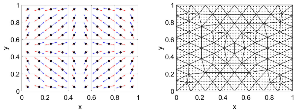
Fig. 12 The exact solution in which particles (marked with dots) move back and forth along the marked vectors (left) and the unstructured grid with the initial particle configuration (right)
