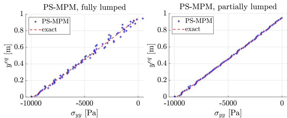
Fig. 18 The equilibrium stress at individual particles in a damped solid column. The numerical solutions were determined with fully lumped and partially lumped PS-MPM at t = 10 s, at which the solution was in equilibrium
