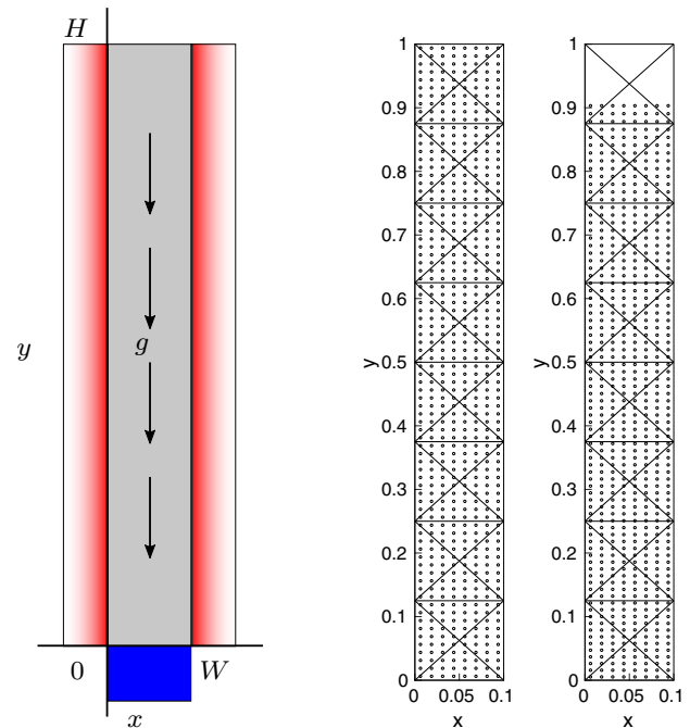
Fig. 16 The column and a discretisation with the expected material point positions at t = 0 and t = 0.186
