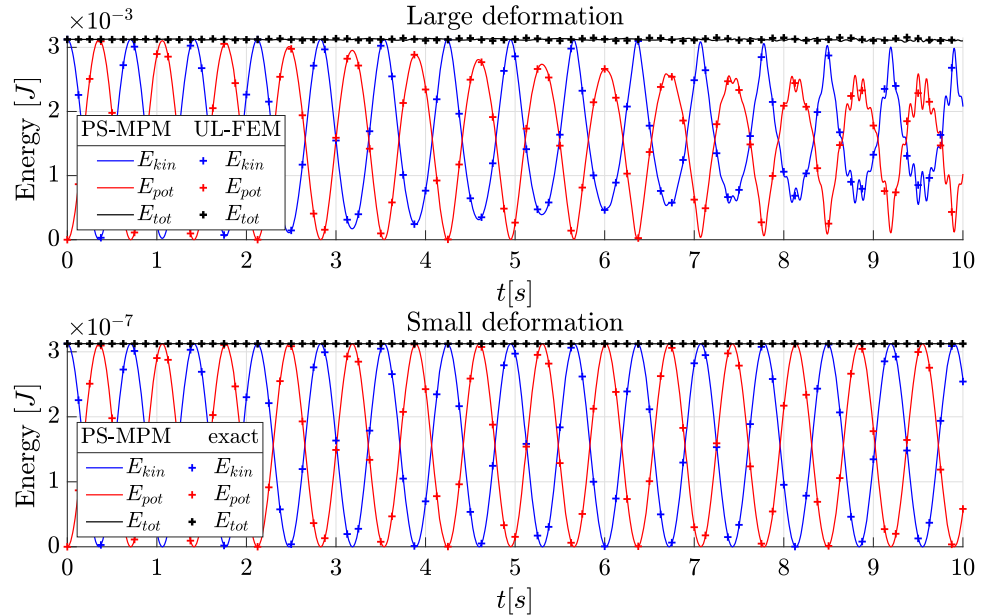
Fig. 11 Energy in the vibrating bar with large deformations (above), and for small deformations (below). Both are compared with a sampled reference solution
