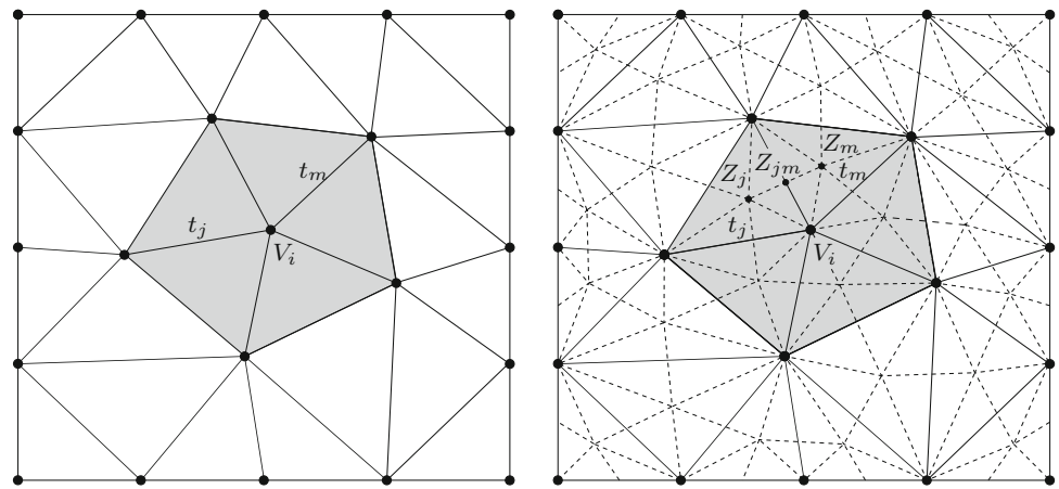
Fig. 2 A triangular grid (left) and a possible PS-refinement (right). The molecule \Omega_i around vertex V_i is marked grey. (Color figure online)
