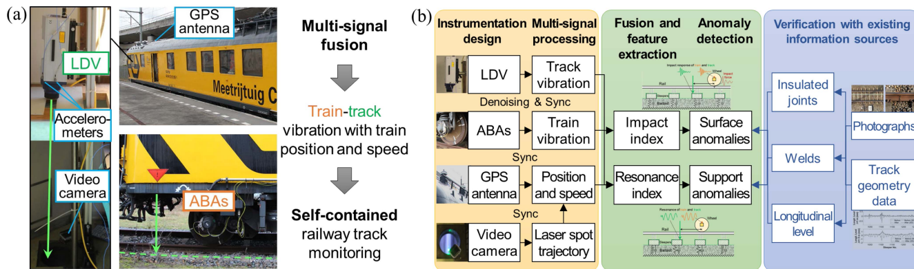
Fig. 1. Train-borne LDV and ABAs with multisignal fusion for self-contained track monitoring. (a) Field implementation. (b) Research framework.
