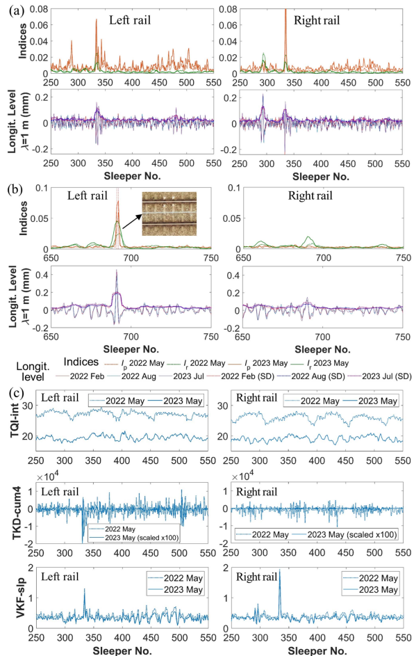
Fig. 13. Other detected anomalies in Section B. (a) Sleeper No. 250–550. (b) Sleeper No. 650–750. “SD” represents the standard deviation of the longitudinal level (source of aerial photographs: ProRail geoinformation portal). (c) Results of Sleeper No. 250–550 following the existing ABA-based methods, in which TQI-int is calculated according to [19], TKD-cum4 is calculated according to [20], and VKF-slp is calculated according to [21].
