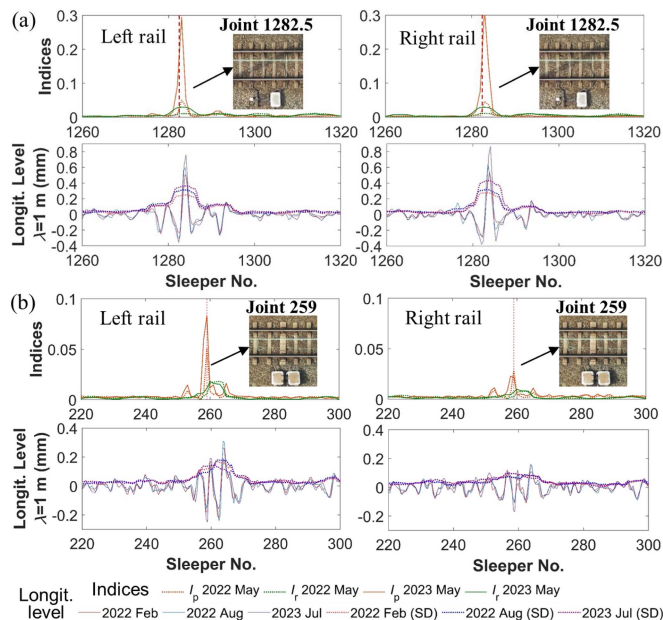
Fig. 11. Indices and longitudinal level near the joints. (a) Joint in Section A. (b) Joint in Section D. “SD” represents the standard deviation of the longitudinal level. (Source of aerial photographs: ProRail geoinformation portal).
