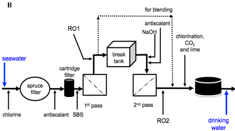
Figure 1.7. KAUST desalination plant (A) segment and (B) scheme of treatment stages. SBS: sodium bisulphite / RO1: seawater reverse osmosis permeate / RO2: brackish water reverse osmosis permeate
