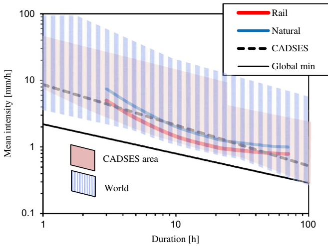
Fig. 9. Range of thresholds collated by Guzzetti et al. (2007) in a) CADSEES area (red) and b) world (striped blue). Thresholds for rail earthworks (red line, thicker) and natural slopes (blue line, thinner); thresholds for CADSEES area (Guzzetti et al., 2007, dashed black line) and global threshold (thin black line Guzzetti et al., 2008) superimposed.
