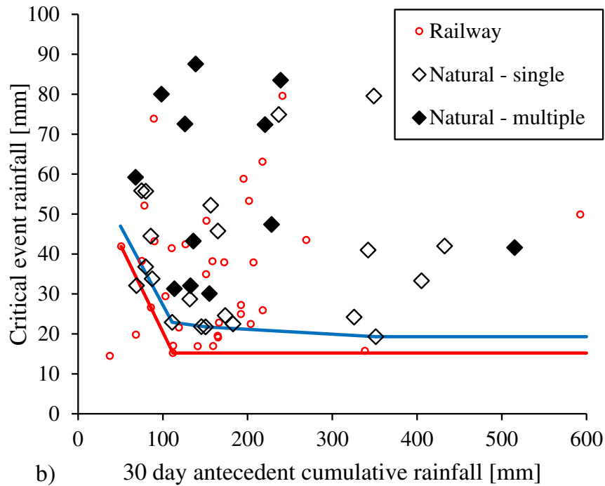
Fig. 8. Cumulative – antecedent rainfall thresholds for landslides on rail network (red line) and landslides on natural terrain (blue line): a) 10 day antecedent period and b) 30 day antecedent period. Landslide events on rail network in red circles. Landslide events on natural terrain in black diamonds. Empty diamond – single landslide event, full diamond – multiple (widespread) landslide event.
