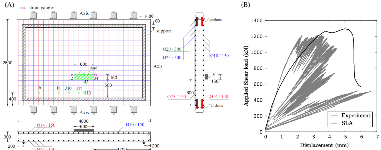
FIGURE 6 (A) Experimental setup of the shear test on reinforced concrete slab: Loading plate, reinforcement layout, and axial load application setup 21 and (B) comparison of the sequentially linear analysis and experimental force displacement curves 13 [Colour figure can be viewed at wileyonlinelibrary.com ]
