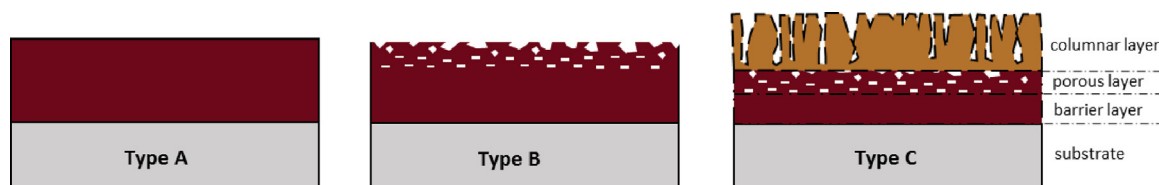
Fig. 10. Different types of morphology observed for the protective layer, based on [11].
