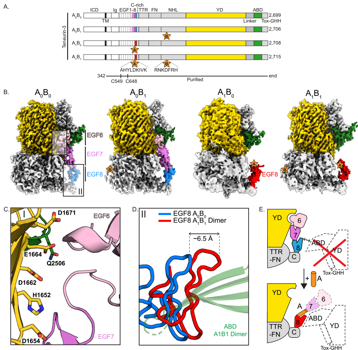
Fig. 4 | Subunits of A_0 isoforms display a contact between EGF6 and the YD/ABD domains. A Linear representations of the four full-length Ten3 isoforms with domain composition. The presence of splice inserts is indicated with stars. Domains are labelled according to Fig. 1. The expressed and purified ectodomain for each isoform is indicated with the black line below. B Cryo-EM reconstructions of isoform subunits (left to right: EMD-18891, EMD-18900, EMD-18902, EMD-18890). Dashed boxes I-II indicate close-ups shown in (C, D), respectively. C EGF6-YD/ABD interface (PDB:8R54). Interacting residues shown on the YD- and ABD-side of the interface
