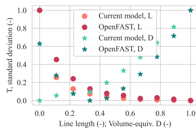
Figure 1: Mooring line tension st. dev. against design variables.
