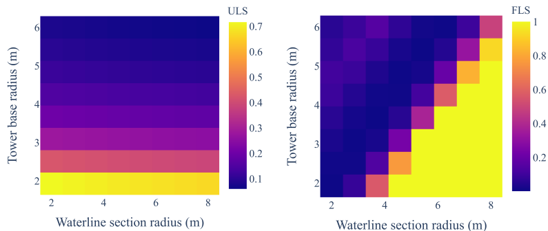
Figure 13: Tower base section strength utilisation.
