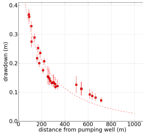
Figure 2-9: Drawdown versus distance to pumping well with 95% confidence intervals for monitoring wells M3, M4, M6 and M7 for all virtual pumping tests; dotted line is best-fit of de Glee
