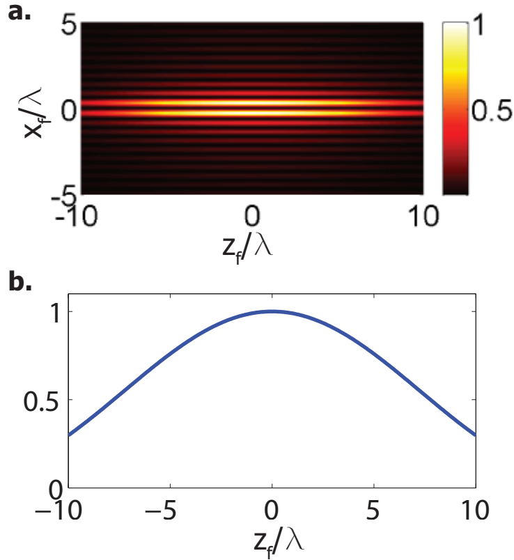
Figure 5: Elongated subwavelength hollow spot by a radially polarized annular aperture with phase vortex m = 1 on the exit pupil, NA=0.99. (a). Normalized focal field distribution in the x_f - z_f plane; (b). Focal intensity distribution along the z_f axis, while x_f is at the maximum intensity on the transversal plane
