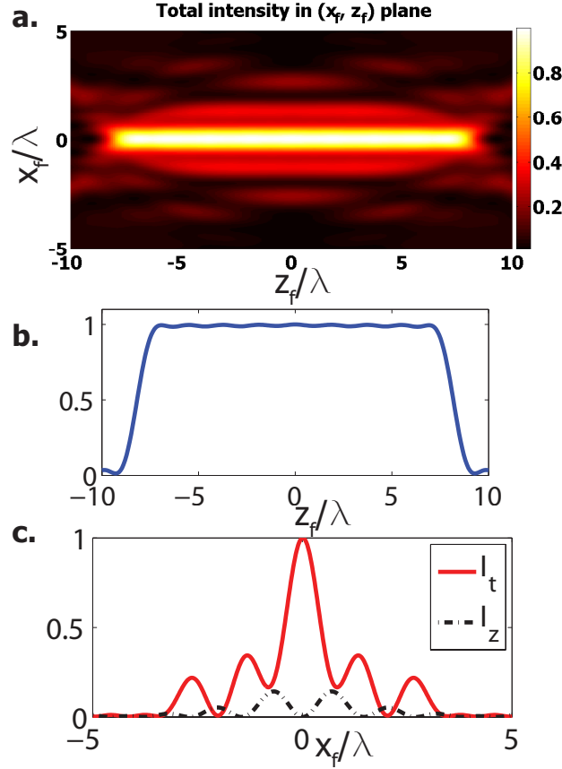
Figure 6: Elongated focal spot with stronger transversal polarisation component by an shaped radially polarized phase vortex with m = 1 on the exit pupil, NA=0.9. (a).Normalized focal intensity distribution in the x_f - z_f plane; (b). Focal intensity distribution along the optical axis; (c). Transversal and longitudinal components of the focal intensity distribution along x_f axis.
