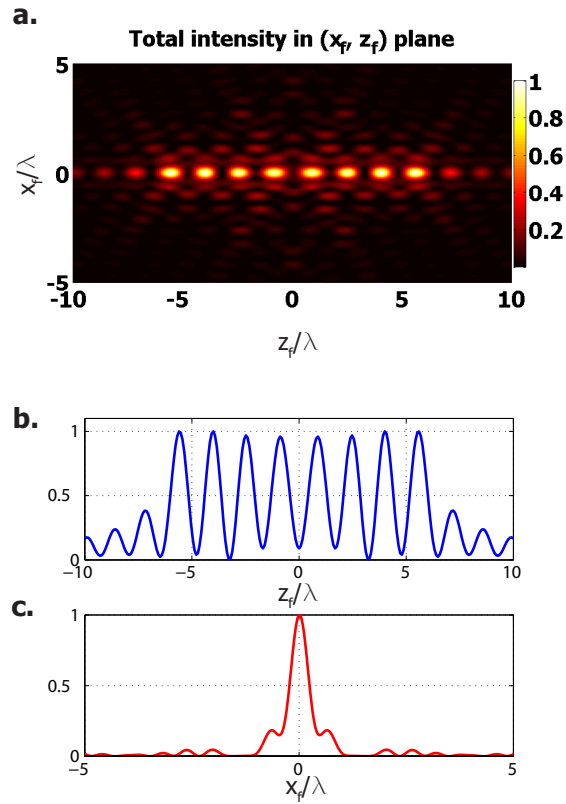
Figure 8: Multiple focal spot along optical axis by an shaped azimuthally polarized phase vortex with m = 1 on the exit pupil, NA=0.99 . (a). Normalized focal field distribution in the (x_f, z_f) plane; (b). Focal intensity distribution along the optical axis; (c). Focal intensity distribution along the x_f axis, z_f is at one of the locations where the spot has maximum on axis intensity.
