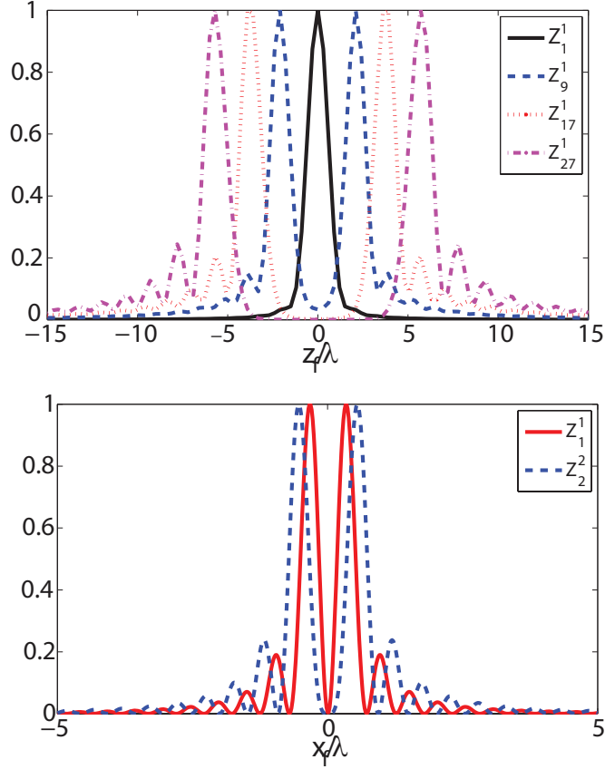
Figure 2: (a). Normalized z -component of the focal intensity for various radially polarized Z_n^1 along z_f axis, lateral position is at its intensity maxima in the transversal plane, the numerical aperture is 0.99. (b). Normalized z -component of the focal intensity for various radially polarized pupil field Z_m^m along x_f axis, z position is at its intensity maxima in the longitudinal plane, the numerical aperture is 0.99.
