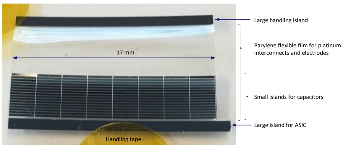
Figure 4.7: Top-view photography of the 80 μm thin released device composed of 128 small (2070 μm x 210 μm) and two large (17 mm x 1 mm and 18 mm x 1 mm) silicon islands separated by 40 μm wide trenches and connected with the 10 μm thick parylene-based flexible interconnect.
