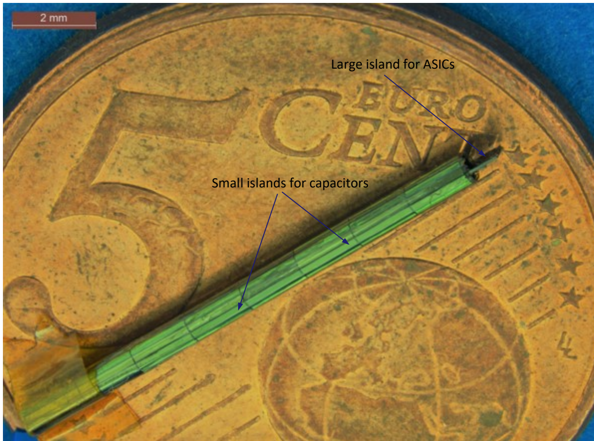
Figure 4.18: The DBS demonstrator wrapped into a cylindrical probe with a length of 18 mm and a diameter of 1.39 mm. The large silicon island for ASICs is wrapped inside the probe.
