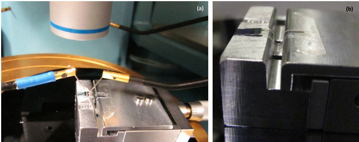
Figure 8.14: (a) The bending tool with a device placed on a probe station during the measurement. (b) Individual device mounted in a bending tool. Sample at an initial bending radius of 1000 \mu\text{m} .
