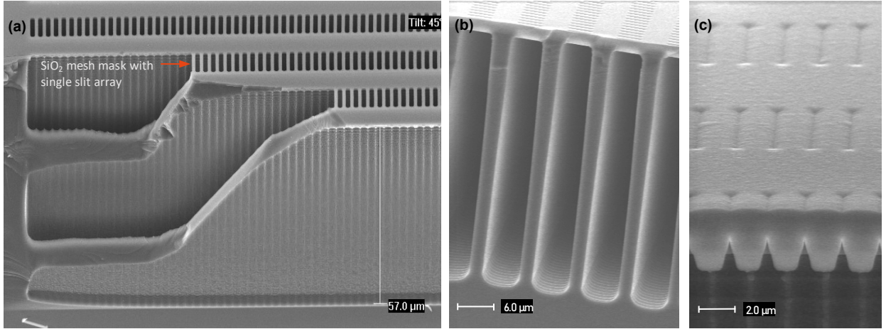
Figure 4.3: SEM image of 6 μm wide and 57 μm deep vertical microchannels etched through an oxide mesh mask in a single-step DRIE process. (a) Cross-section through channels with preserved thin silicon dioxide mesh mask. (b) Cross-section through a row of parallel channels after sealing them with PECVD SiO 2 . (c) Cross-section through sealing of an embedded channel.
