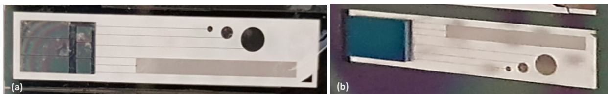
Figure 7.6: Fabricated semi-flexible device with parylene-platinum based interconnects, platinum electrodes, and a rigid silicon island with bond pads. (a) Front side of the wafer. (b) Backside of the wafer.
