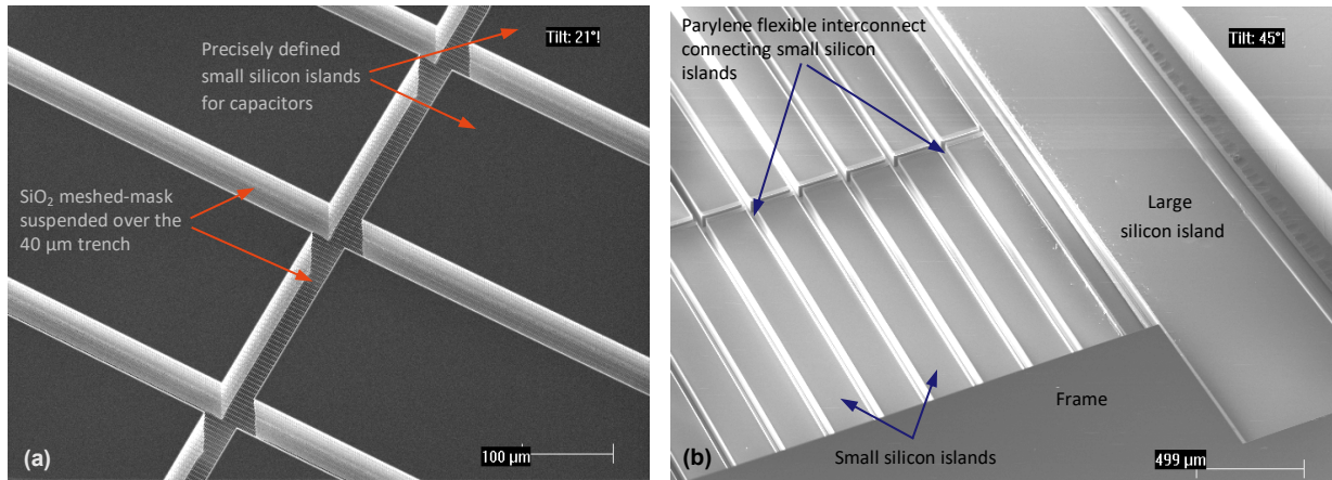
Figure 4.6: SEM images of the precisely defined 80 μm thick silicon islands. (a) Top view of the remaining SiO 2 mesh-shaped mask after the trench front-side DRIE process. (b) Bottom view of the final device with separated small and large silicon islands after the back-side two-step DRIE release.
