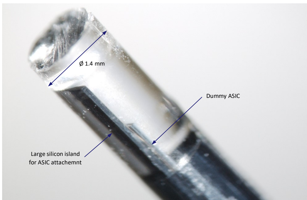
Figure 5.6: The mock-up DBS device filled with medical-grade epoxy EPO-TEK MED-301-2FL. Source: FIZM.
