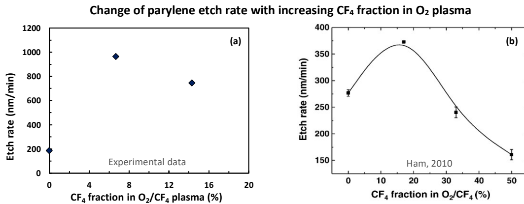
Figure 6.14: The change in parylene etch rate related to the addition of \text{CF}_4 to the \text{O}_2 plasma in the RIE process. (a) Experimental data. (b) Data collected by Ham, 2010 [19].
