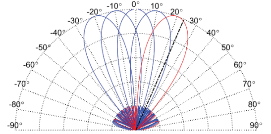
Fig. 3. MIMO-monopulse scan by generating multiple beams simultaneously. Target is at 23 degrees within the red beam steered to 20 degrees
