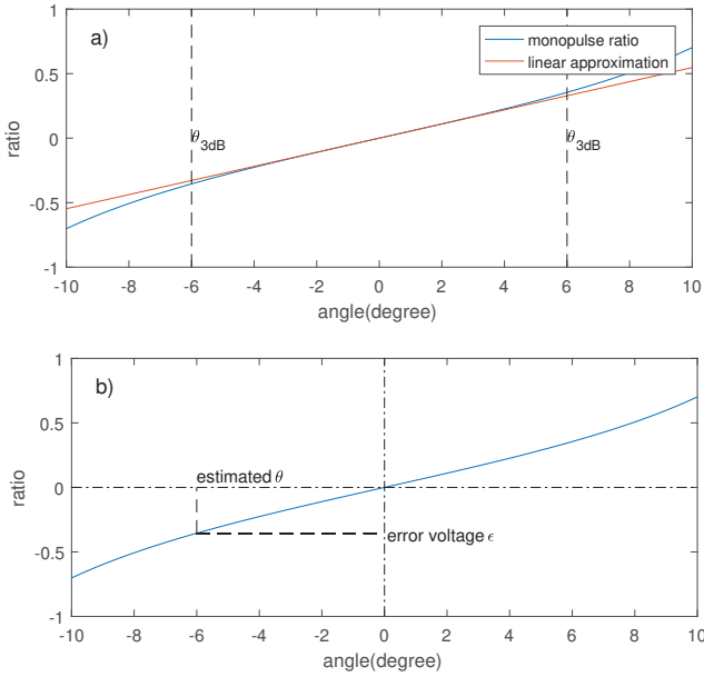
Fig. 2. (a) Monopulse ratio and linear approximation ; (b) Error voltage and inverse mapping
