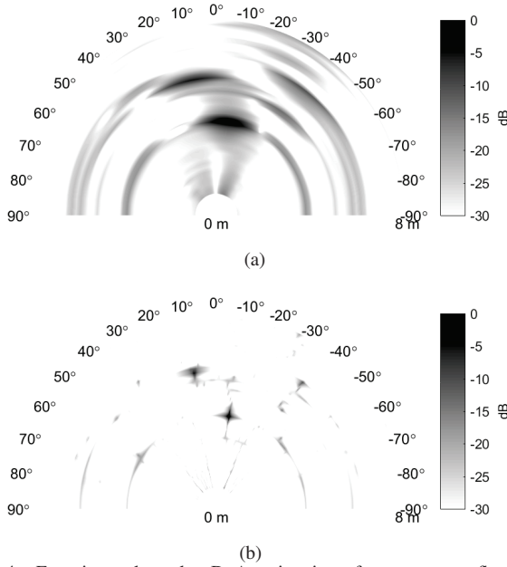
Fig. 4. Experimental results: DoA estimation of two corner reflector in an indoor environment by a) DBF, b) MIMO-monopulse.
