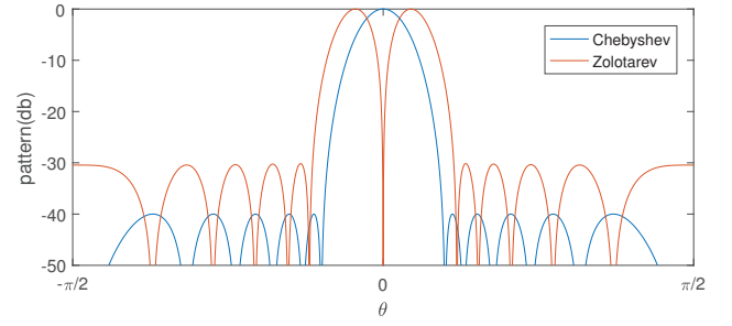
Fig. 1. Sum (Chebyshev) and difference (Zolotarev) beam pattern of the proposed synthesis
