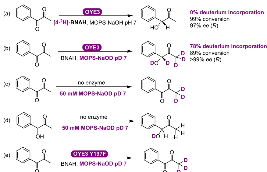
Figure 5. OYE3-catalyzed monoreduction of 7a to 7b with (a) dideuterated cofactor [4-^2\text{H}] -BNAH in buffer (50 mM MOPS-NaOH pH 7.0); (b) BNAH in deuterated buffer (50 mM MOPS-NaOD pD 7.0); (c, d) control reactions without enzyme; (e) reaction with OYE3 Y197F. Conditions: 60 \mu\text{M} OYE3, 30 mM 1-phenyl-1,2-propanedione, 30 mM cofactor, 4.5 h at 30 ^\circ\text{C} , anaerobic.
