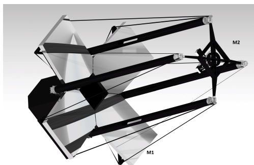
Figure 3.1: Artistic impression of the TU Delft Deployable Space Telescope.
