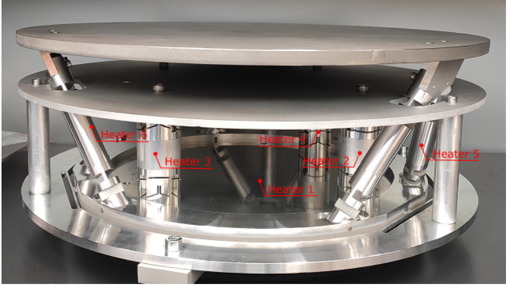
Figure 4.8: Picture indicating where the flexible heaters were attached to the setup.
