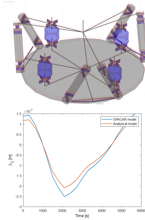
Figure 3.17: Deviation over time caused by thermal fluctuations of the flexure joints (case 1). Top figure displays the case shape, the bottom figure shows computed piston values with SPACAR and analytical models.
