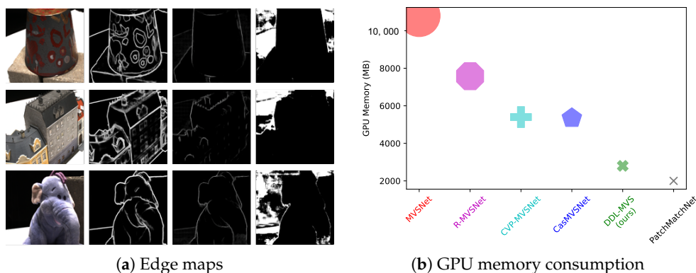
Figure 4. Edges maps and GPU Memory consumption. (a) Edges maps of a few randomly chosen examples. For each example, the images from left to right are the color image, the edge map predicted by HED [60], our learned edge map, and the \alpha map, respectively. We can see that our learned edge maps better capture the depth discontinuities, regardless of the photometric changes. It is also interesting to observe that our \alpha maps distinguish between foreground and background. (b) Comparison of GPU memory demands with existing learning-based MVS networks on DTU dataset with image size 1152 \times 864 .
