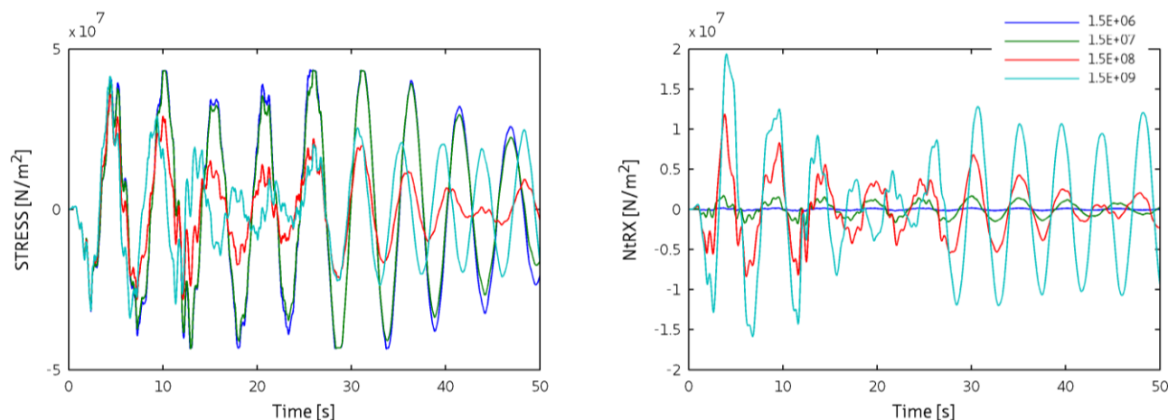
Fig. 8 - Stress distribution per damping coefficient of the dampers ( \alpha=0.5 ) in the core (left) and perimeter columns (right) under scaled El Centro
