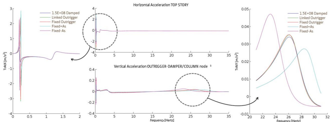
Fig. 7 – Accelerations responses versus frequency of top story and node Outtrigger-Damper/Column for different structural arrays of the 60-s building with outrigger
