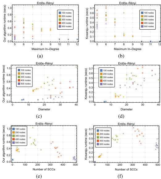
Fig. 4. Relationship between the network properties of some randomly generated Erdős–Rényi networks and their run-times for both our proposed algorithm and Kossaraju’s algorithm.
