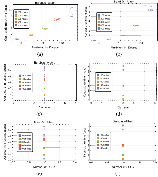
Fig. 6. Relationship between the network properties of some randomly generated Barabási–Albert networks and their run-times for both our proposed algorithm and Kossaraju’s algorithm.
