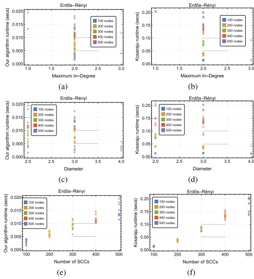
Fig. 2. Relationship between the network properties of some randomly generated Erdős–Rényi networks and their run-times for both our proposed algorithm and Kossaraju’s algorithm.
