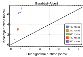
Fig. 7. Run-times of both our proposed algorithm and Kosaraju's algorithm for several randomly generated Barabási–Albert networks. We see that our algorithm performs better on networks with a higher number of nodes.
