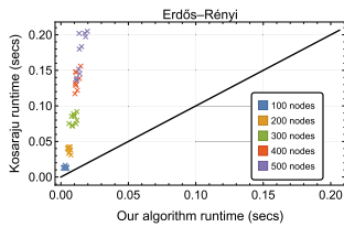
Fig. 3. Comparison of the run-times of both our proposed algorithm and Kossaraju’s algorithm for several randomly generated Erdős–Rényi networks. We see that our algorithm performs better on networks with a higher number of nodes.
