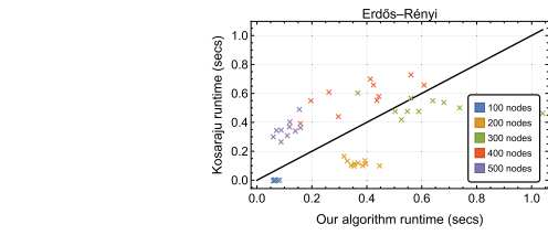
Fig. 5. Comparison of the run-times of both our proposed algorithm and Kossaraju’s algorithm for several randomly generated Erdős–Rényi networks. We see that our algorithm performs better on networks with a higher number of nodes.
