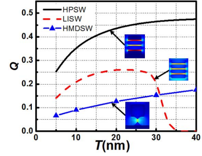
Fig. 3. Dependence of the confinement factor ( Q ) for HPSWs, LISWs and HMDSWs with the thickness of \text{SiO}_2 layer ranging from 5 to 40 nm.
