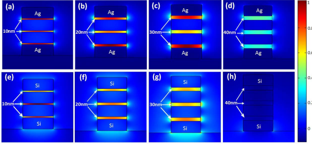
Fig. 2. The cross-section of the electrical field distributions for both HPSWs [(a)-(d)] and LISWs [(e)-(h)] with different thickness of \text{SiO}_2 layers at 10 nm, 20 nm, 30 nm, and 40 nm, respectively.
