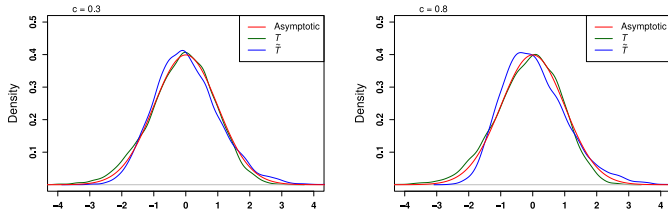
Fig. 2. The high-dimensional asymptotic normal approximation of the densities of T_\alpha and \tilde{T}_\alpha together with their kernel density estimators for \gamma = 5 , p = 300 and c_n = p/n \in \{0.3, 0.8\} .
