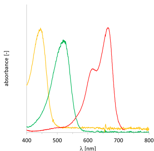
Figure 1. Coverage of the visible light spectrum by combining flavin mononucleotide (orange), phenosafranin (green), and methylene blue (red).
