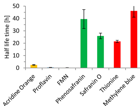
Figure 5. Stability of the photocatalysts upon illumination. General conditions: 100 \mu\text{M} photocatalysts, 50 mM KPi buffer, pH 7, 300 rpm, 30 ^{\circ}\text{C} .
