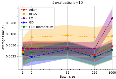
Figure 2: Evaluation speed per batch size, with \mu = 10 , lr = 0.001 , and no clipping. The scale of both axes is logarithmic. Lines are median values over the 10,000 trees of the experiment described in Sec. 3.1, and shaded areas indicate interquartile ranges.
