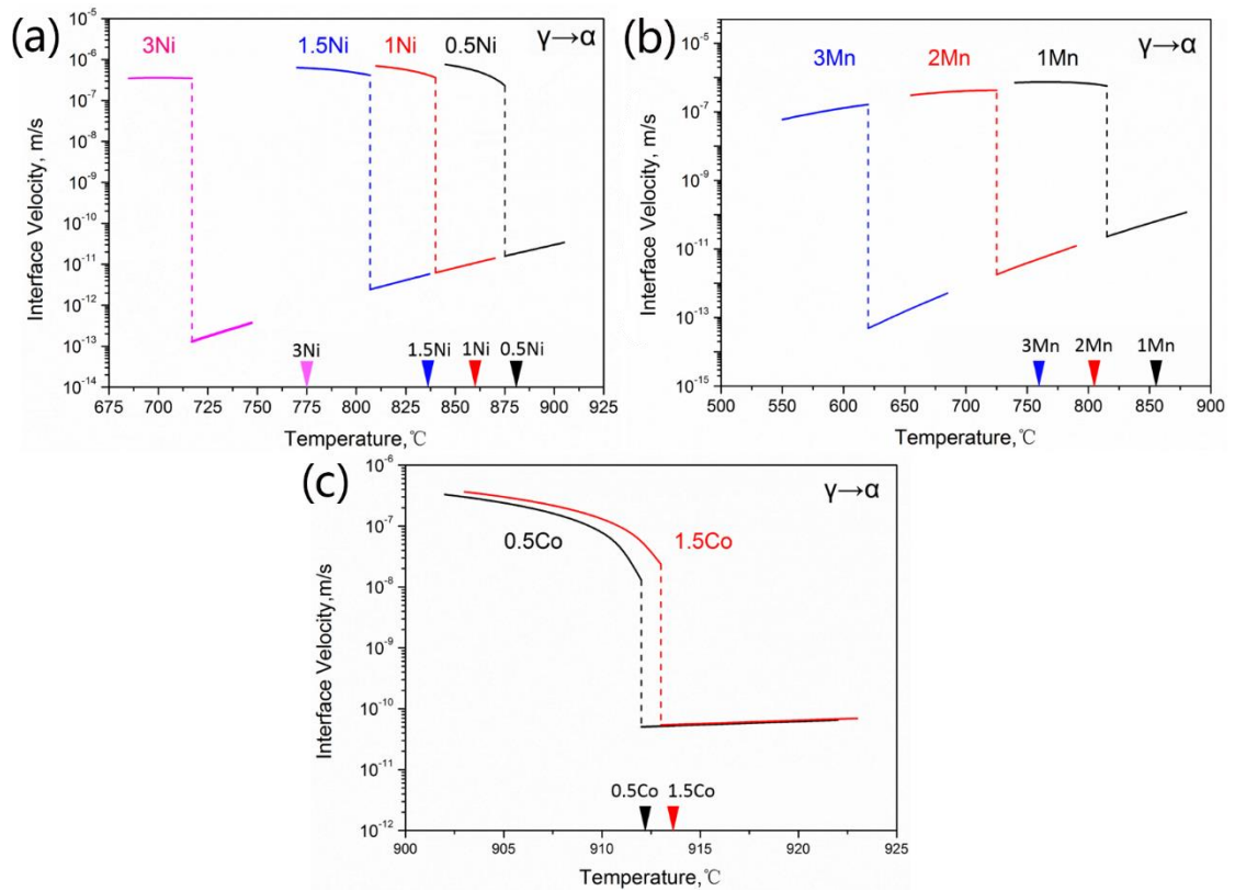
Fig. 9 The predicted interface velocities as a function of temperature for the \gamma \rightarrow \alpha transformation in (a) Fe-Ni (b) Fe-Mn and (c) Fe-Co alloys. The corresponding T_0 temperatures are labelled with the solid arrows
