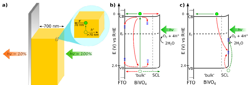
Figure 4. For solid films, there is a trade-off between light-harvesting efficiency and charge separation efficiency (a). Band diagrams of \text{BiVO}_4 showing stepwise processes toward water splitting with (b) light-harvesting and charge separation ( \phi_{\text{sep}} ) followed by (c) charge injection ( \phi_{\text{inj}} ). The green paths support water splitting, whereas the red paths are loss pathways.
