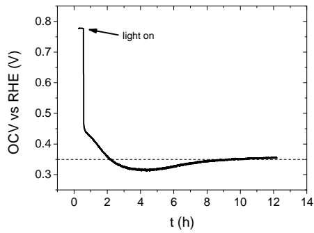
Fig. S4. Open circuit potential of BiVO 4 photoanode immersed in 0.1 M PBA buffer pH 10 under AM1.5G simulated illumination.
