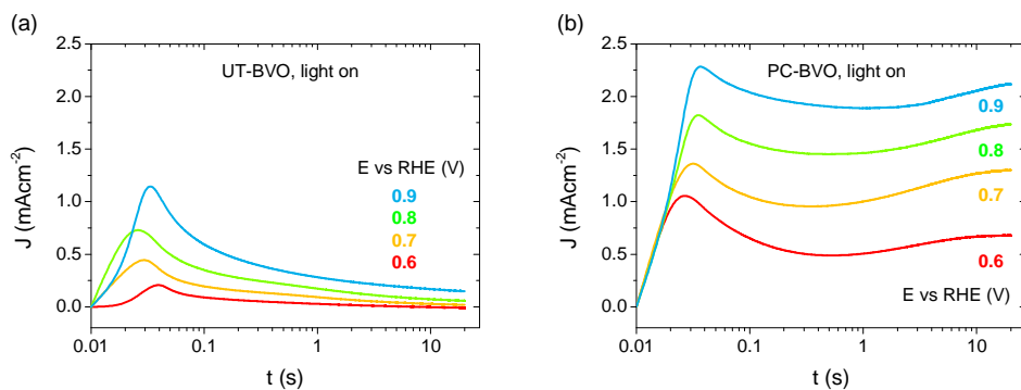
Fig. S14. Anodic transients of an (a) untreated and (b) photocharged BiVO 4 photoanode immersed in 0.1 M PBA buffer pH 10, under AM1.5G simulated illumination and at applied bias of 0.6, 0.7, 0.8 and 0.9 V vs RHE.
