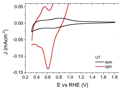
Fig. S12. Cyclic voltammetry of untreated (UT) \text{BiVO}_4 in the dark and under illumination. Zoom in of Figures 6 (a) and (b) combined.
