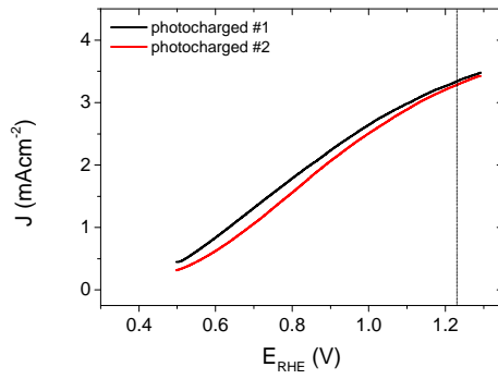
Fig. S2 The JV performance of a photocharged \text{BiVO}_4 photoanode (black), which was subsequently left in the cell for 24 h to discharge under dark conditions and recharged back again (red).
