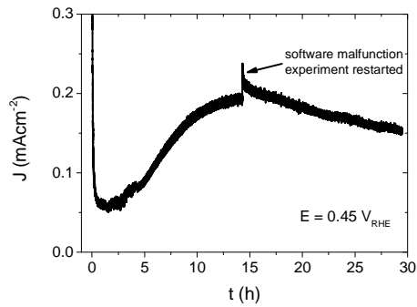
Fig. S5. Chronoamperometry measurement of BiVO 4 photoanode held at 0.45 V_{RHE} , 0.1 V more anodic vs the reference OC potential, subsequent to Fig. S7.
