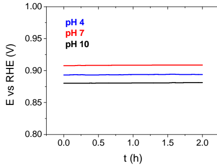
Fig. S3. Steady state OC potentials of BiVO 4 photoanodes collected in the dark and in various pHs.
