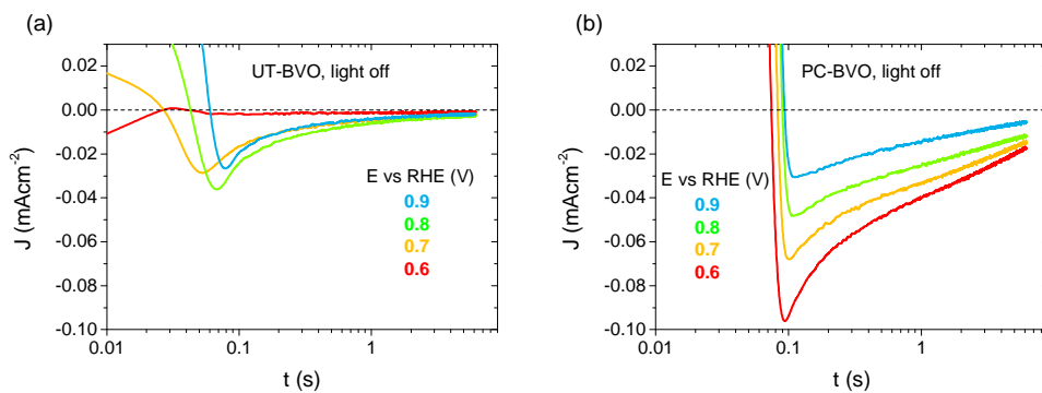
Fig. S15. Cathodic transients of an (a) untreated and (b) photocharged BiVO 4 photoanode immersed in 0.1 M PBA buffer pH 10, in the dark and at applied bias of 0.6, 0.7, 0.8 and 0.9 V vs RHE.
