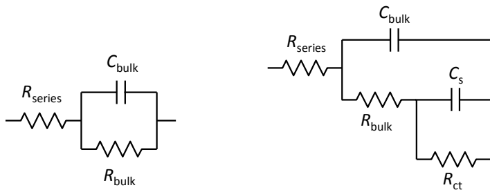
Fig. S13. Equivalent circuit used to fit impedance spectroscopy data of BiVO 4 in the dark (left), and under illumination (right).
