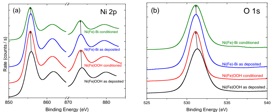
Fig. S5. Collected XPS spectra for as deposited and conditioned samples of Ni(Fe)-Bi and Ni(Fe)OOH. (a) Ni2p and (b) O1s orbital scans.
