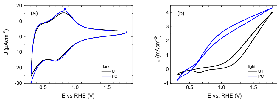
Figure 6. Cyclic voltammetry of untreated (UT) and photocharged (PC) \text{BiVO}_4 (a) in the dark and (b) under illumination.
