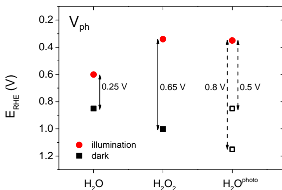
Figure 4. Equilibrium potentials and photovoltage values of \text{BiVO}_4 photoanodes in the open circuit configuration: untreated sample in 0.1M K-P i electrolyte ( \text{H}_2\text{O} ), in presence of a hole scavenger ( \text{H}_2\text{O}_2 ), photocharged sample ( \text{H}_2\text{O}^{\text{photo}} ).
