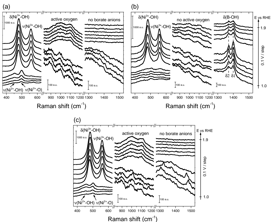
Figure 3. SER spectra of freshly prepared Ni(Fe)(OH) 2 acquired in the potential range 1.0-1.9 V vs RHE in: (a) 0.1 M KOH pH 13, (b) 0.5 M K-B, pH 9.2 and (c) 0.1 M KOH + 0.01 M H 3 BO 3 . The measurements were performed potentiostatically.
