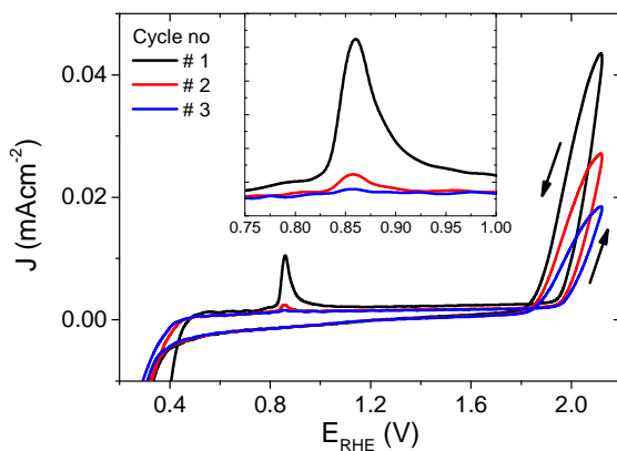
Figure 5. The first three dark JV scans of the BiVO 4 photoanode after 10 hours of photocharging, inset: a zoomed in plot around the observed oxidation peak at \sim 0.85 V RHE .
