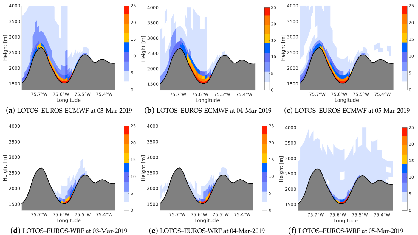
Figure 13. Aburrá Valley vertical profiles. (a–c) The vertical and surface PM_{2.5} daily mean for a high-concentration period using meteorology from ECMWF in LOTOS–EUROS at latitude 6.255^\circ N on 3–5 March. (d–f) The same for WRF data on the same days.
