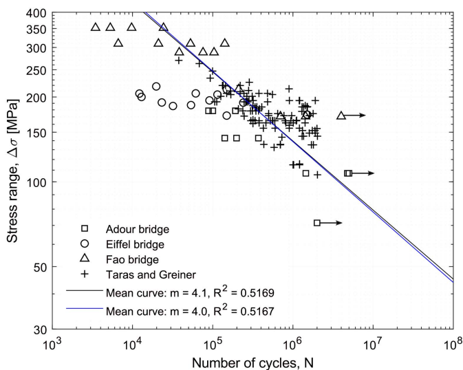
Fig. 6. Experimental data for double riveted connections: mean S-N curves.
