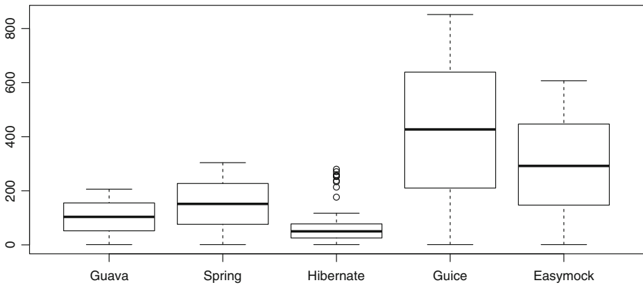
Fig. 6 Lag time distribution in days, by API
