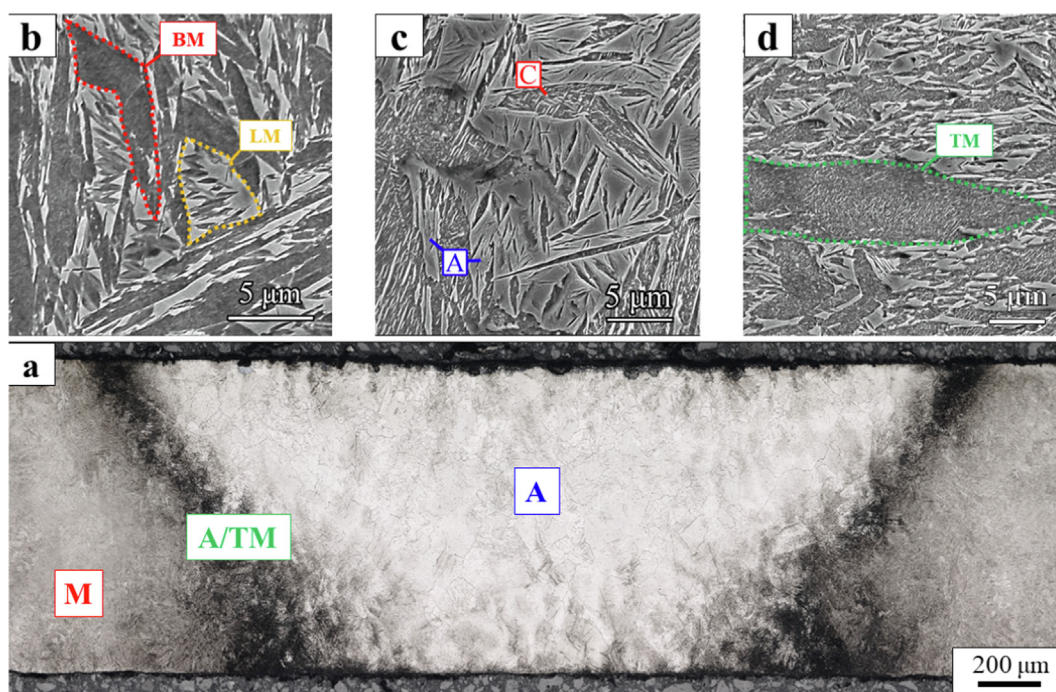
Fig. 3. (a) Cross section of the laser affected zone in martensite one line base material. (b)(c)(d) Magnified SEM micrographs of (b) Martensite base microstructure, (c) A/TM region in (a), and (d) tempered martensite microstructures. M = martensite, TM = tempered martensite, BM = butterfly martensite, LM = lenticular martensite, A = austenite, C = carbides.
