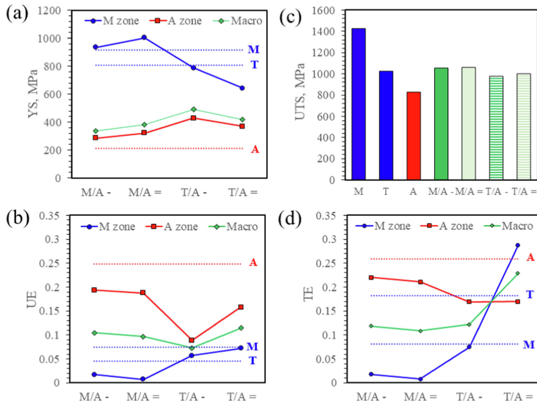
Fig. 6. Comparative mechanical properties of different specimens (Macro) with that measure for individual phases at austenite ( A_{zone} ) and martensite ( M_{zone} ) zones by DIC. (a) Yield strength (YS), (b) uniform elongation (UE), (c) ultimate tensile strength (UTS) and (d) total elongation (TE). Dashed lines represent the properties of reference austenite (A), martensite (M) and tempered martensite (T).
