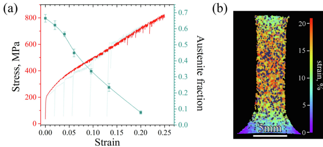
Fig. 5. (a) Engineering stress–strain curve of austenite (in red) represented along with the phase fraction of austenite with strain (green solid symbols) The line present in the figure is presented purely as a reading guide and does not imply a precise fit. The light green stress–strain curve corresponds to the interrupted tests at different strains for XRD measurements. (b) Local strain along the tensile test specimen gauge of the austenite base specimen for a frame of digital image correlation corresponding with 0.2 strain.
