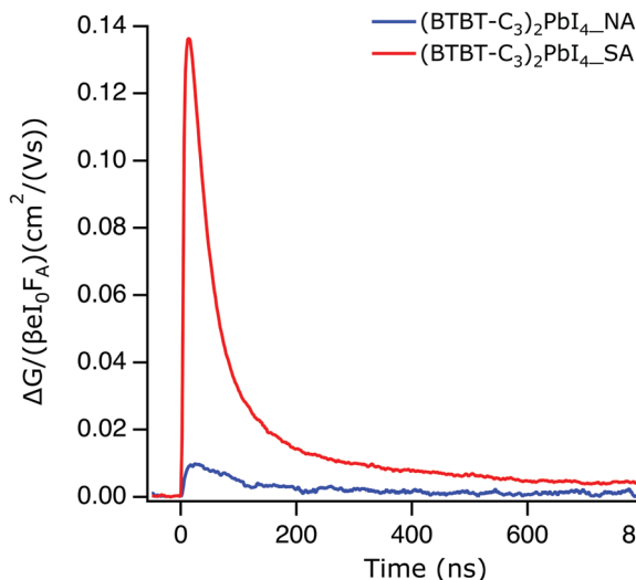
Fig. 12 Photoconductivity TRMC of (\text{BTBT-C}_3)_2\text{PbI}_4 thermal evaporated films (NA) and solvent vapour annealed films (SA). The films were excited at \sim 490 nm with a photon intensity of 4.3 \times 10^{12} ph \text{cm}^{-2} (concentration of \sim 1014 \text{cm}^{-3} ).
