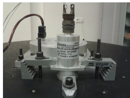
Figure 1. Angular accelerometer type SR-207RFR.
